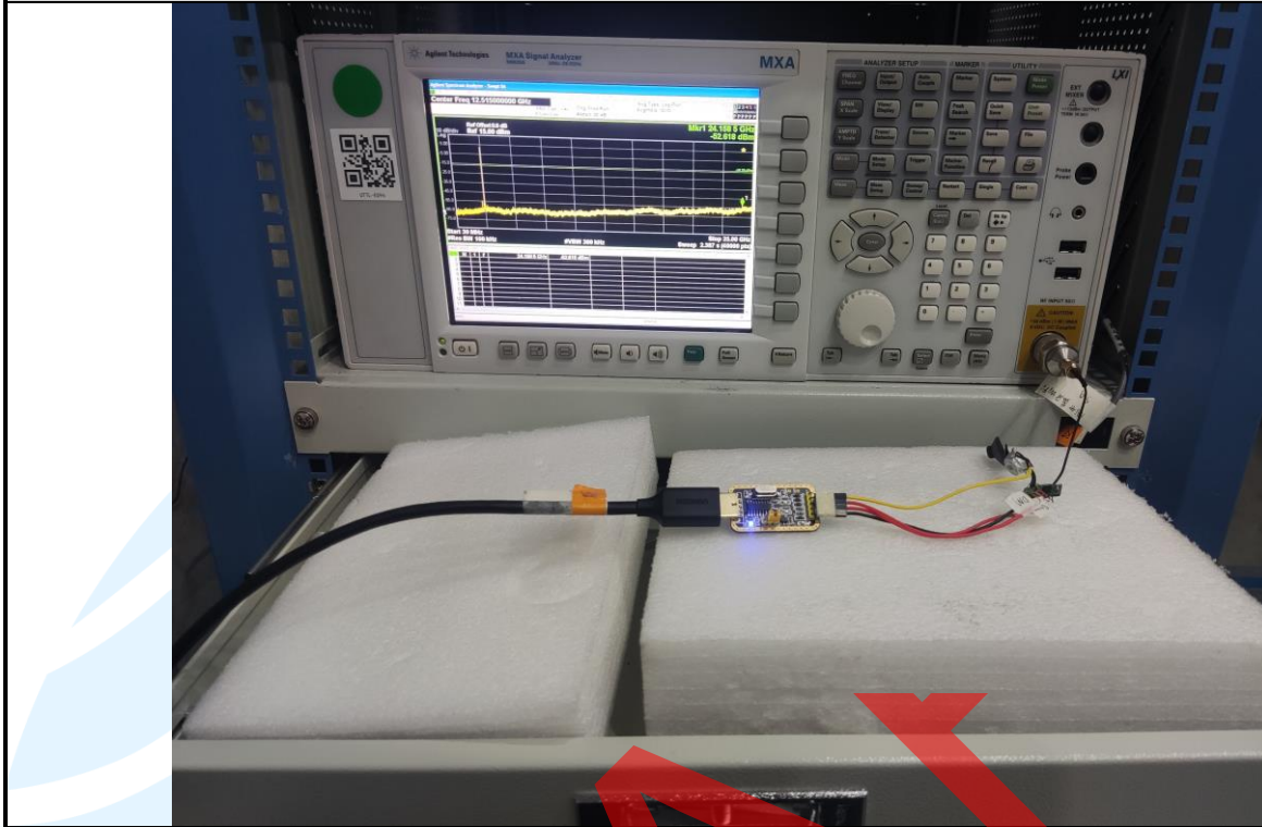
RF Conducted Test Setup_Left earbud
