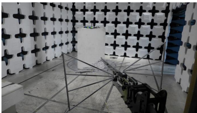
Figure 1: P10T Transmitter Test Setup
