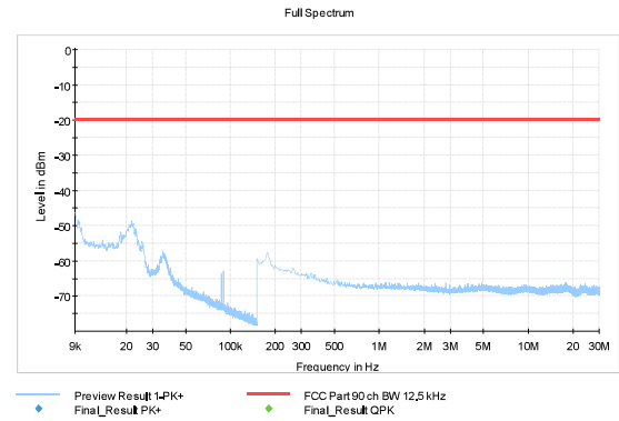
Figure 177: RX 450.5 MHz, 12.5 kHz, GMSK
