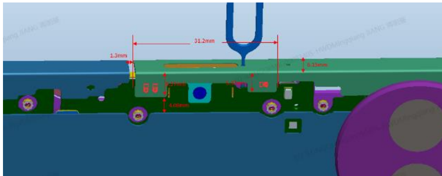
P-sensor coexisted with WLAN 2.4GHz antenna
