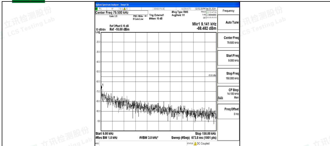
Band41_20MHz_16QAM_40620_1RB#0_0.009~0.15_0.009~0.15
