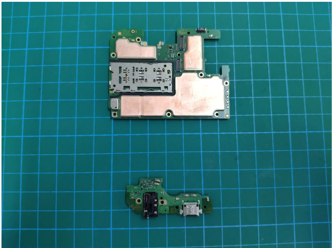
PCB 05:
