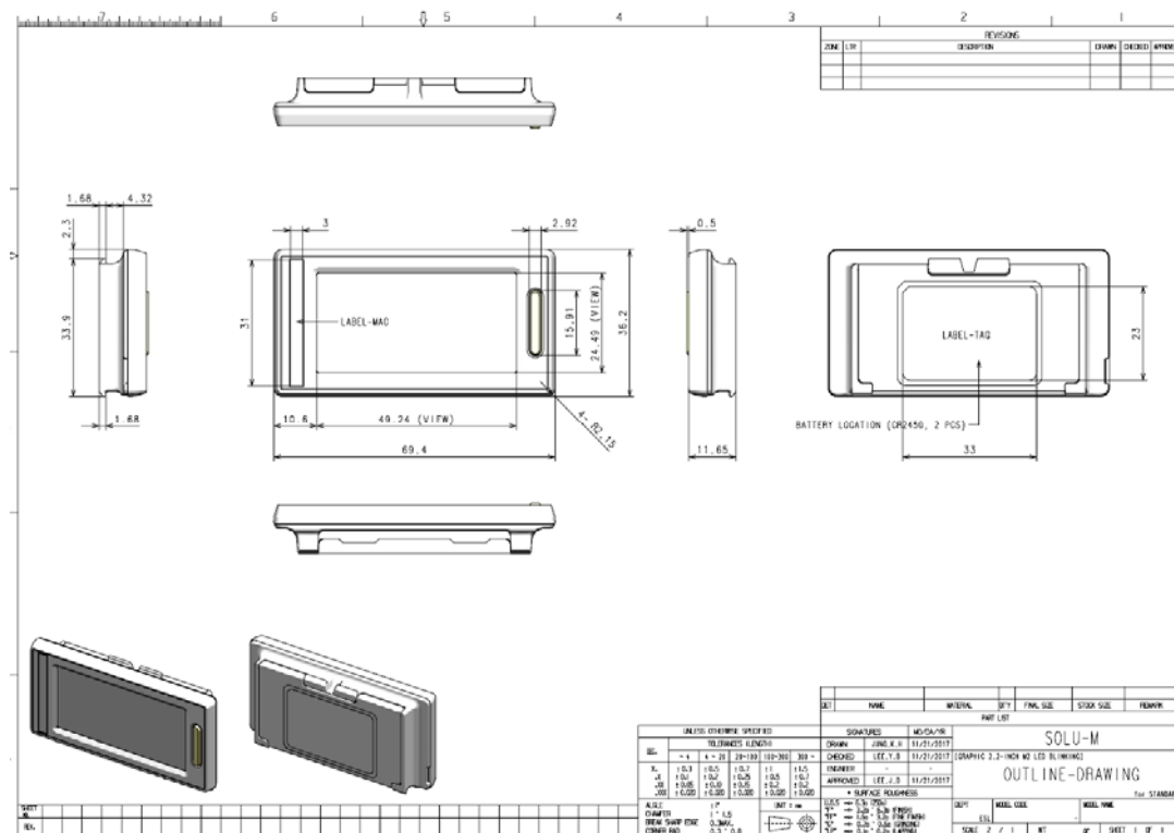
Figure 4. 2.2"Mechanical Dimension
