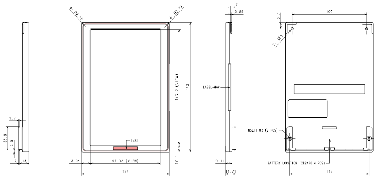
Figure 6.7.4"Mechanical Dimension
