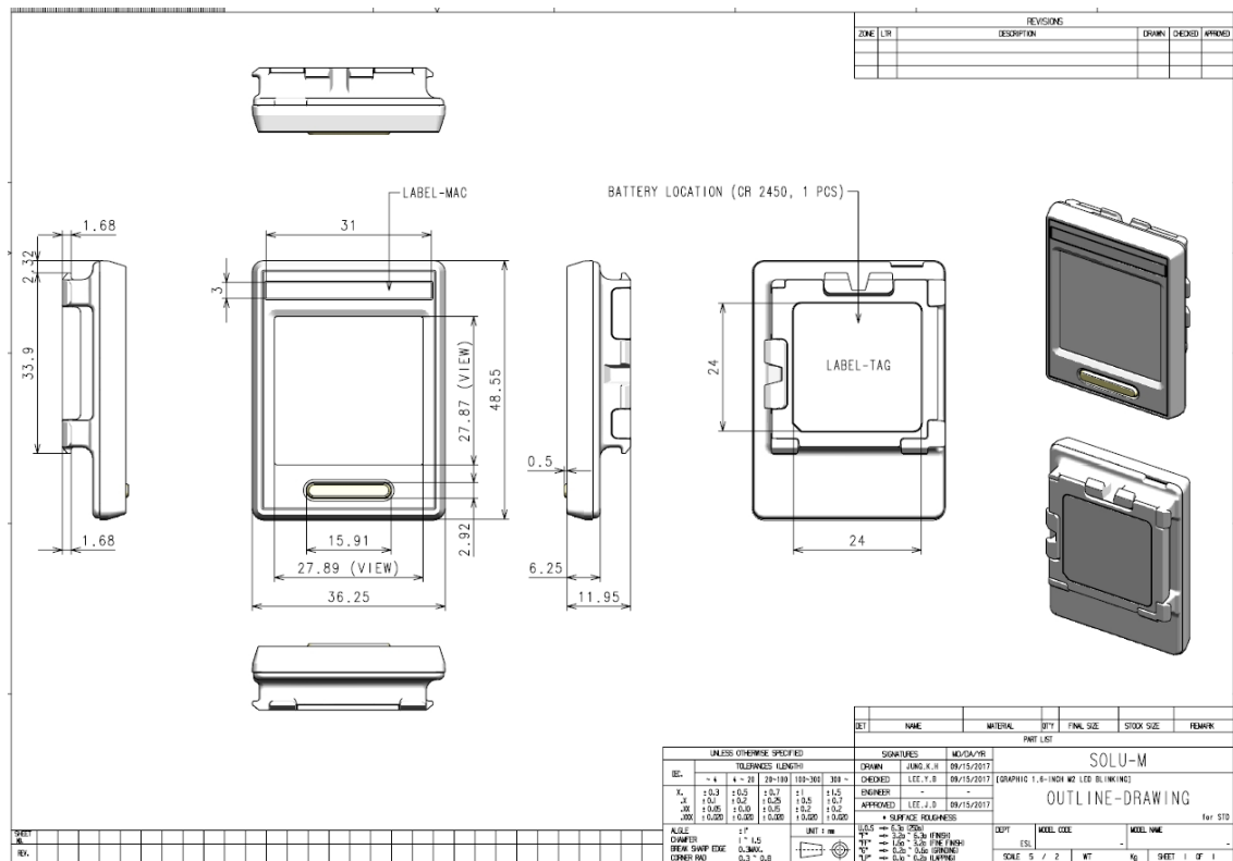
Figure 3 1.6"Mechanical Dimension
