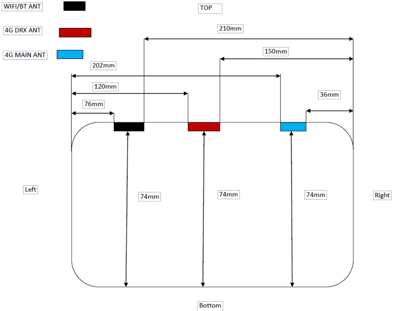
Front View
