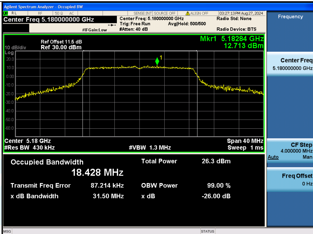
11N20MIMO-Ant3-5180
