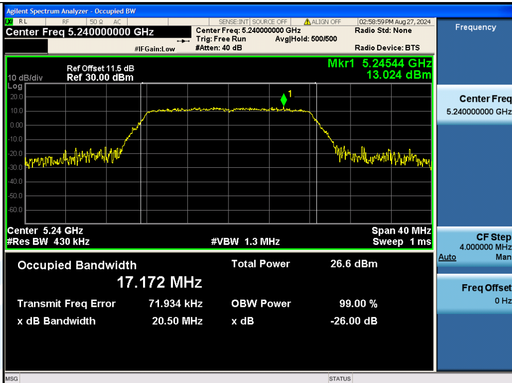
11A-Ant3-5240
