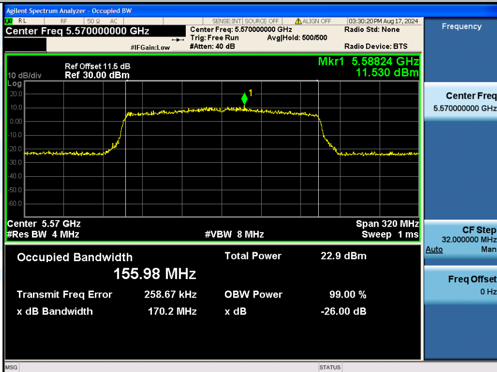
11AX160MIMO-Ant2-5570
