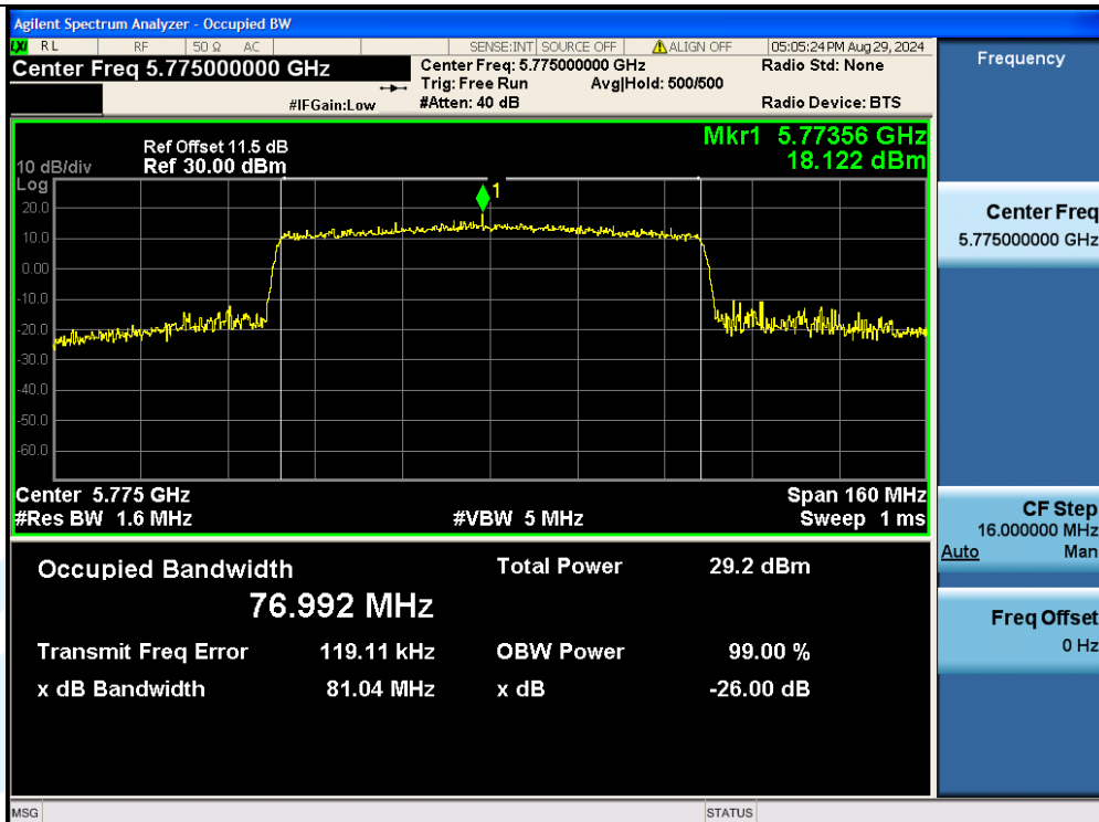
11AX80MIMO-Ant2-5775
