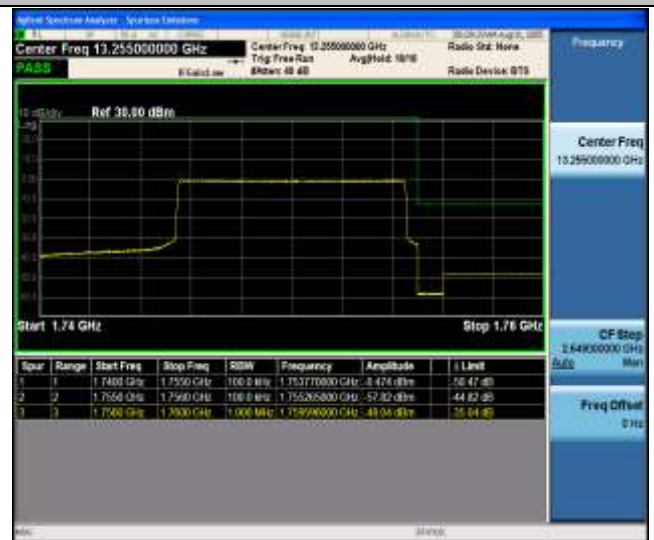
Band4_10MHz_QPSK_20350_50RB#0
