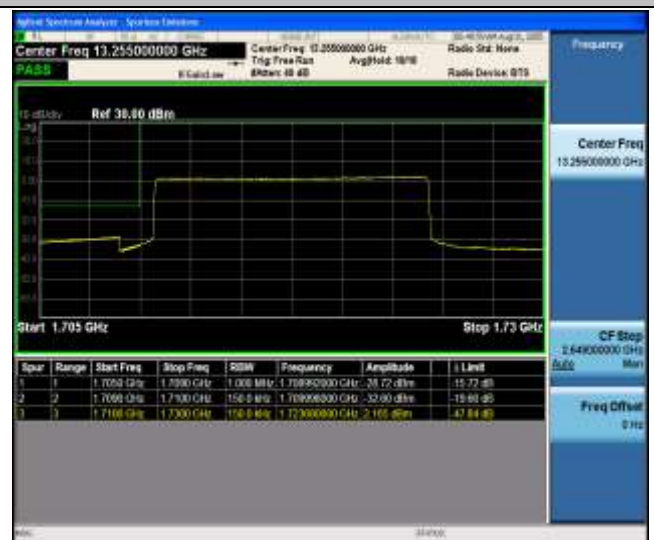
Band4_15MHz_QPSK_20025_75RB#0
