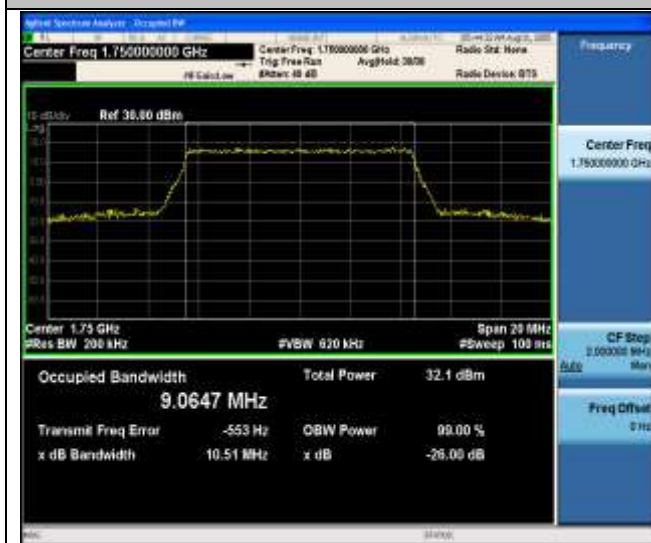
Band4-10MHz-QPSK-20350-50RB#0-PASS
