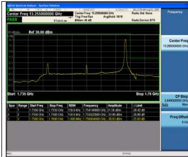
Band4_15MHz_QPSK_20325_1RB#74
