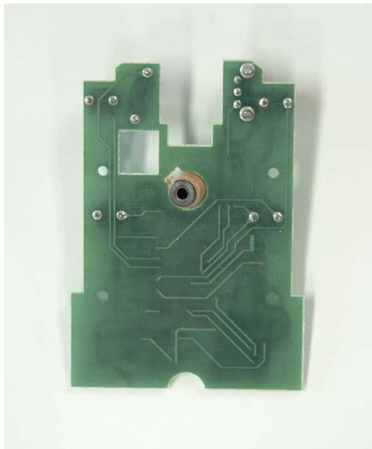
Photo A-19 Reverse of internal board _ 2D Mouse (model: ZC-100)
