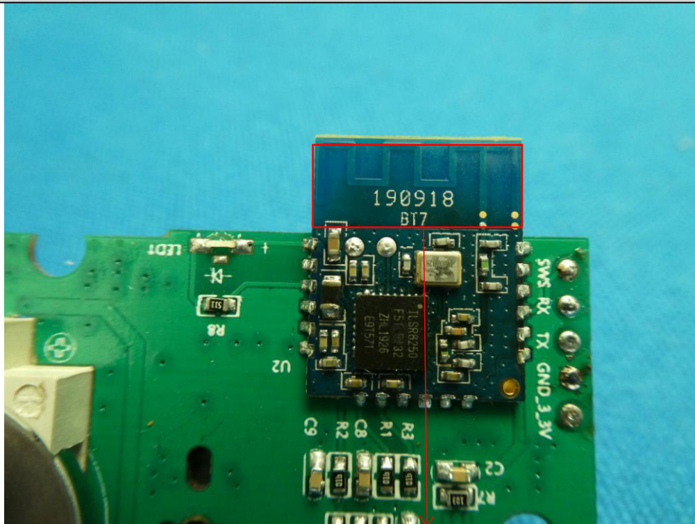
RF Antenna
