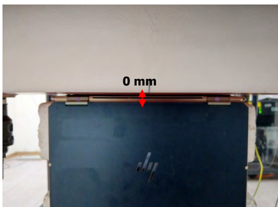
Fig.8 EUT Bottom side (Laptop mode) to flat phantom
