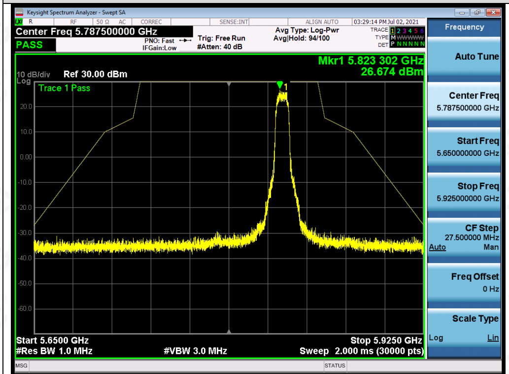
Test_Graph_OFDM_ANT1_5825_MCS0_Frequency Band3
