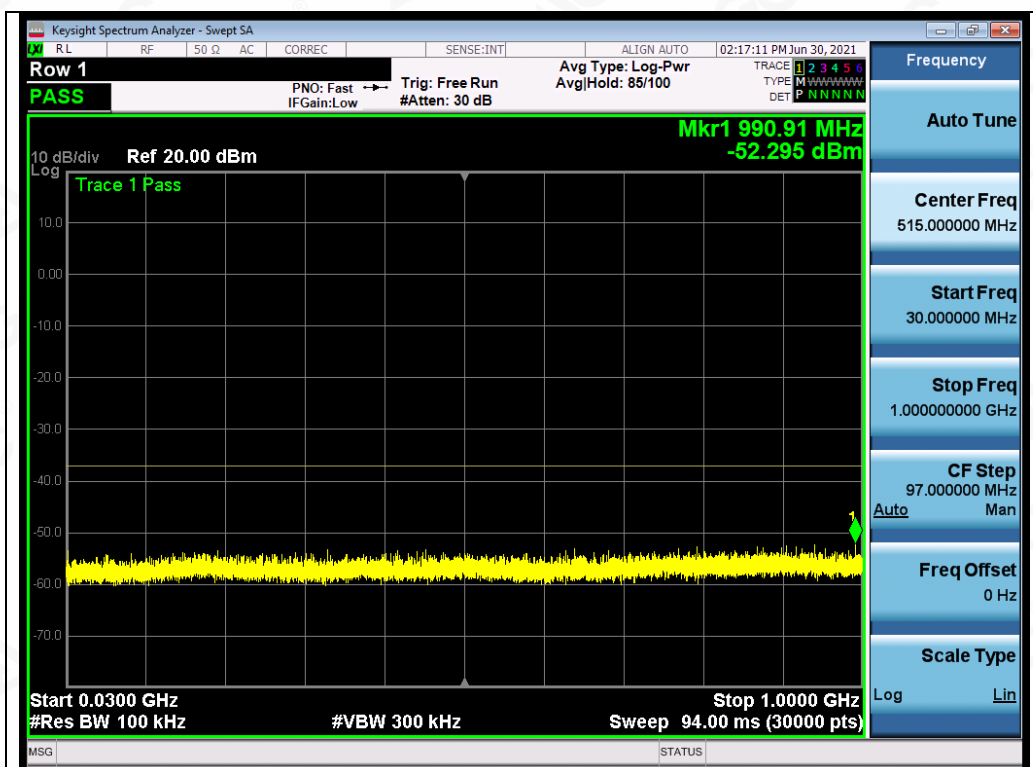
Test_Graph_OFDM_ANT1_5745_6Mbps_Frequency Band1
