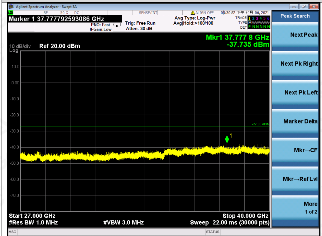
Test_Graph_OFDM_ANT1_5825_6Mbps_Frequency Band5
