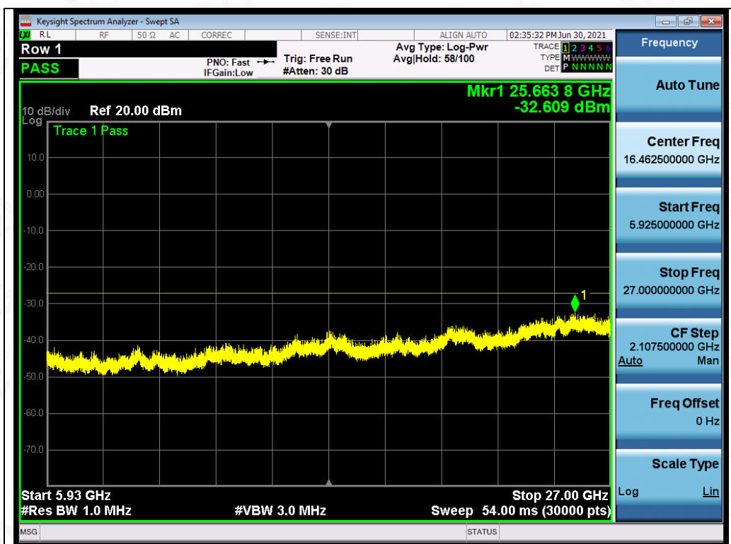
Test_Graph_OFDM_ANT1_5825_6Mbps_Frequency Band4
