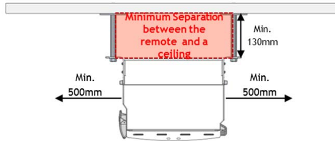
Figure 4.3 – Horizontal Installation
