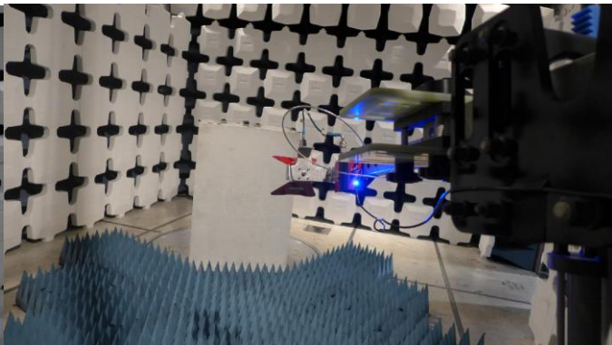
Figure 2: ULXD6 Transmitter Test Setup
