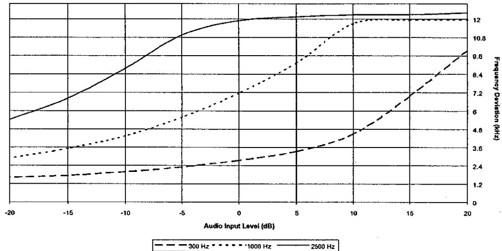
Modulation Limiting Response (Positive Peak)
