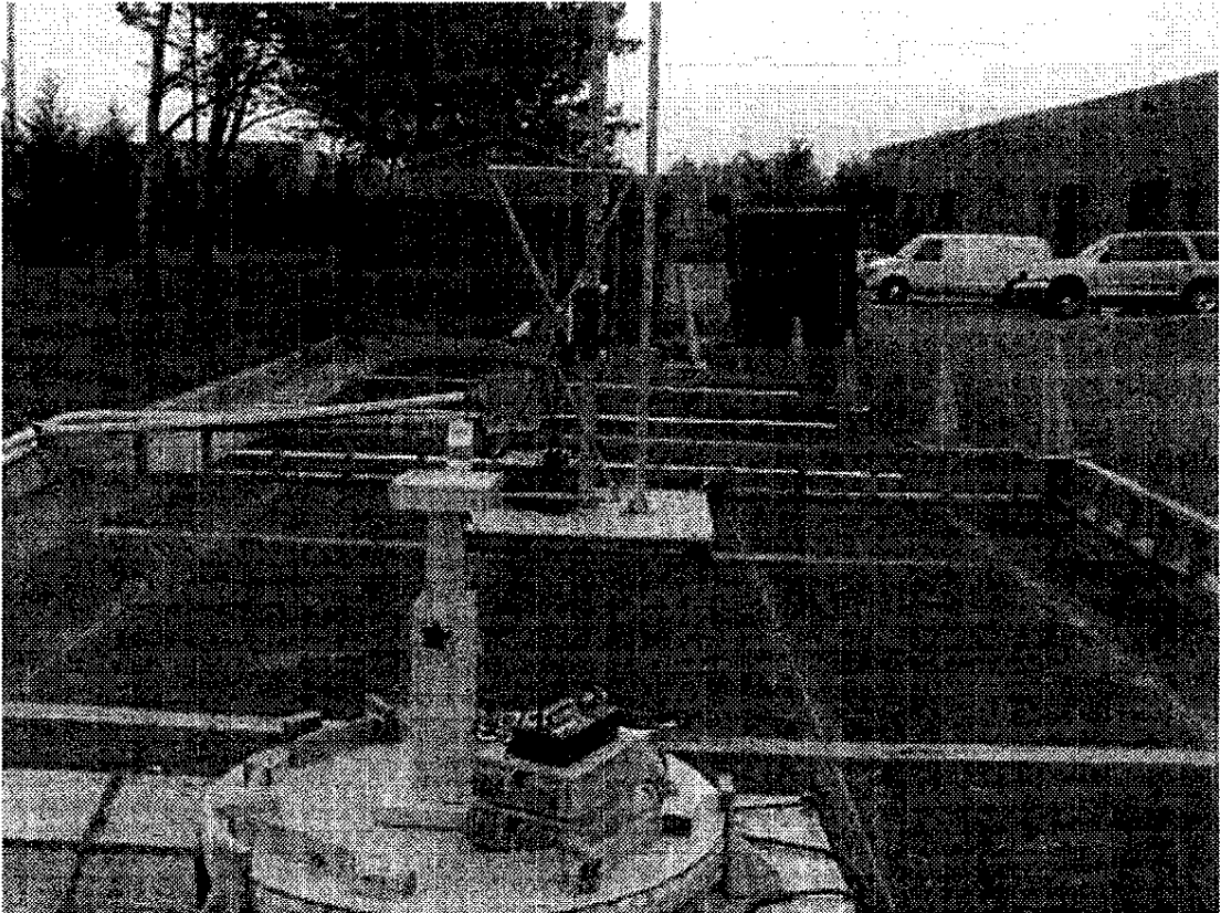
PHOTOGRAPH 1: FRONT VIEW OF RADIATED EMISSIONS
