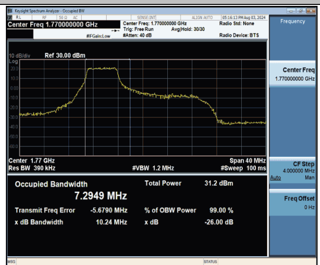
Band66-20MHz-16QAM-132572-27RB#0-PASS
