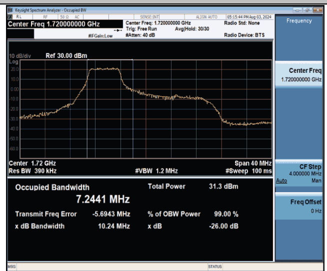
Band66-20MHz-16QAM-132072-27RB#0-PASS
