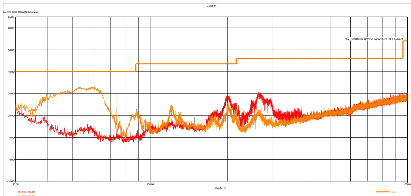
Figure 5 - Radiated Emissions Plot, BTBR, Low Channel
