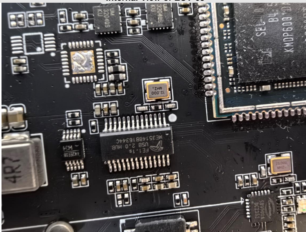
Internal View of EUT-63
