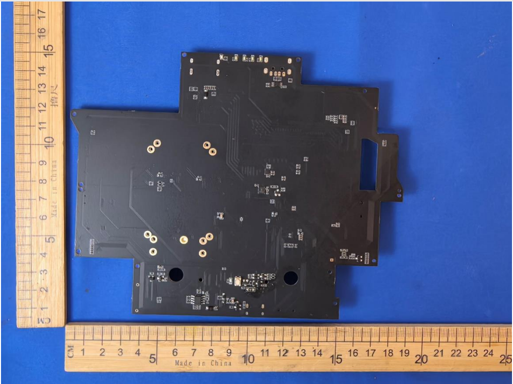
Internal View of EUT-57
