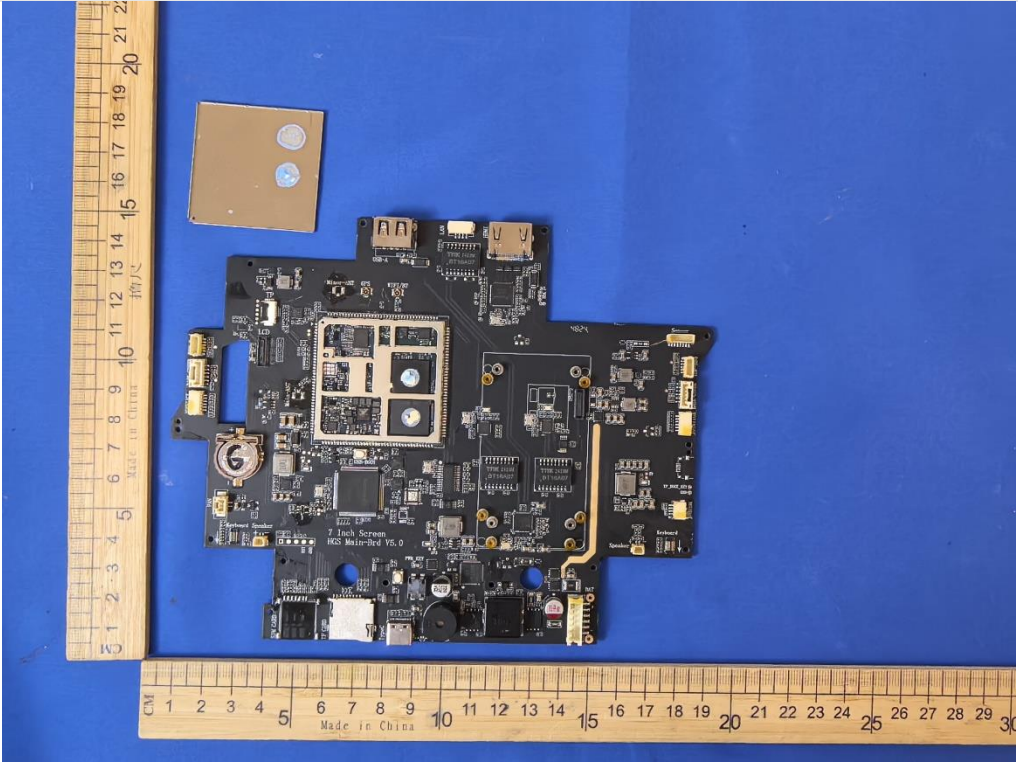
Internal View of EUT-58
