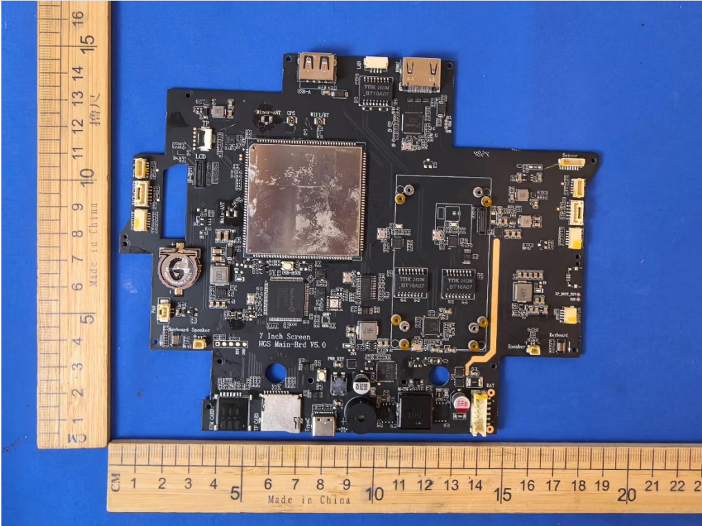
Internal View of EUT-56
