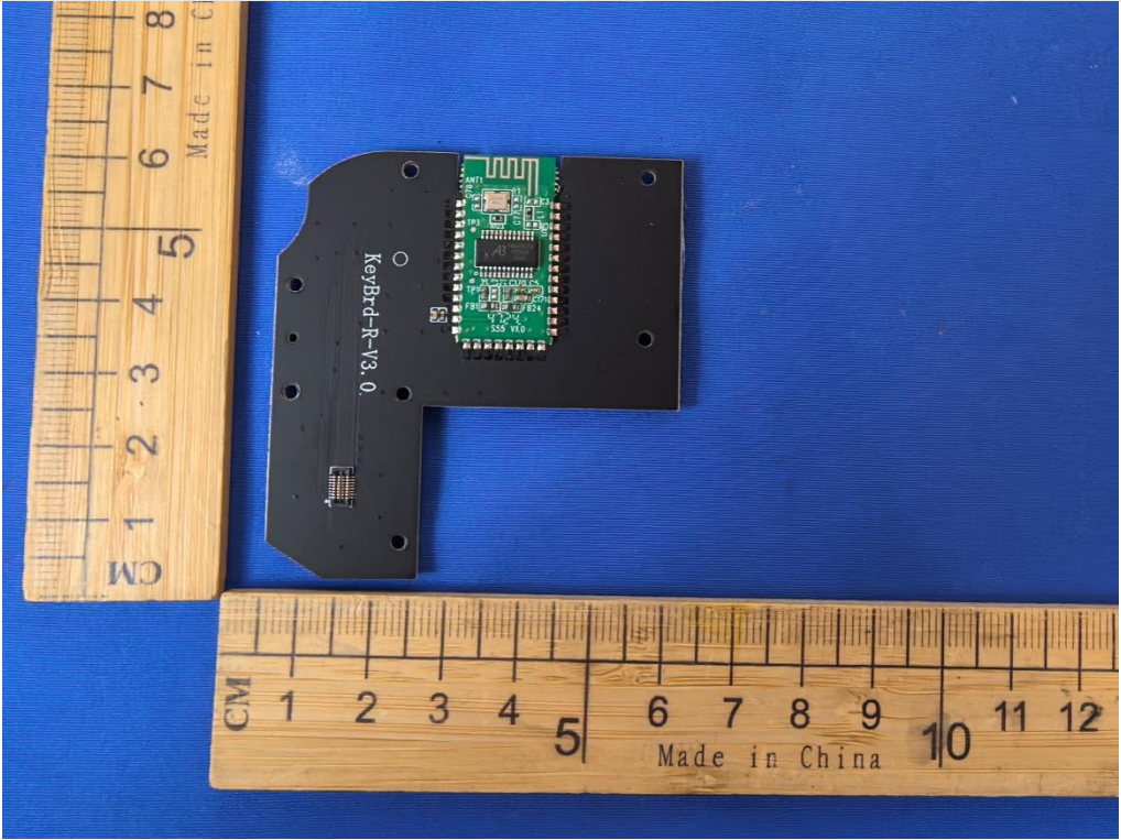
Internal View of EUT-52
