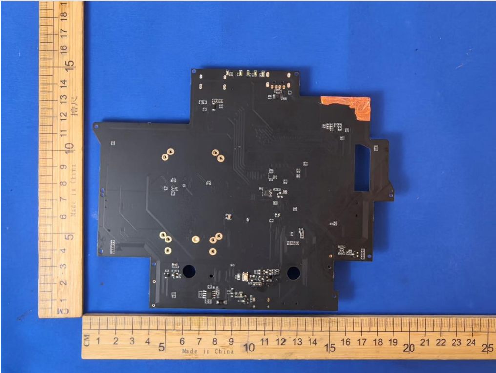
Internal View of EUT-55
