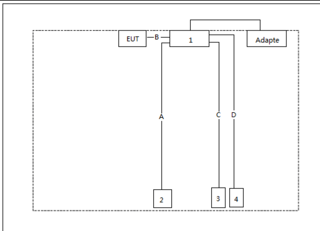
Connection Diagram
