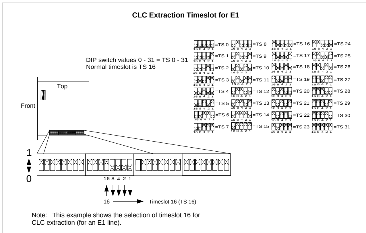
Figure 4-29. Setting the CLC Extraction Timeslot for E1
