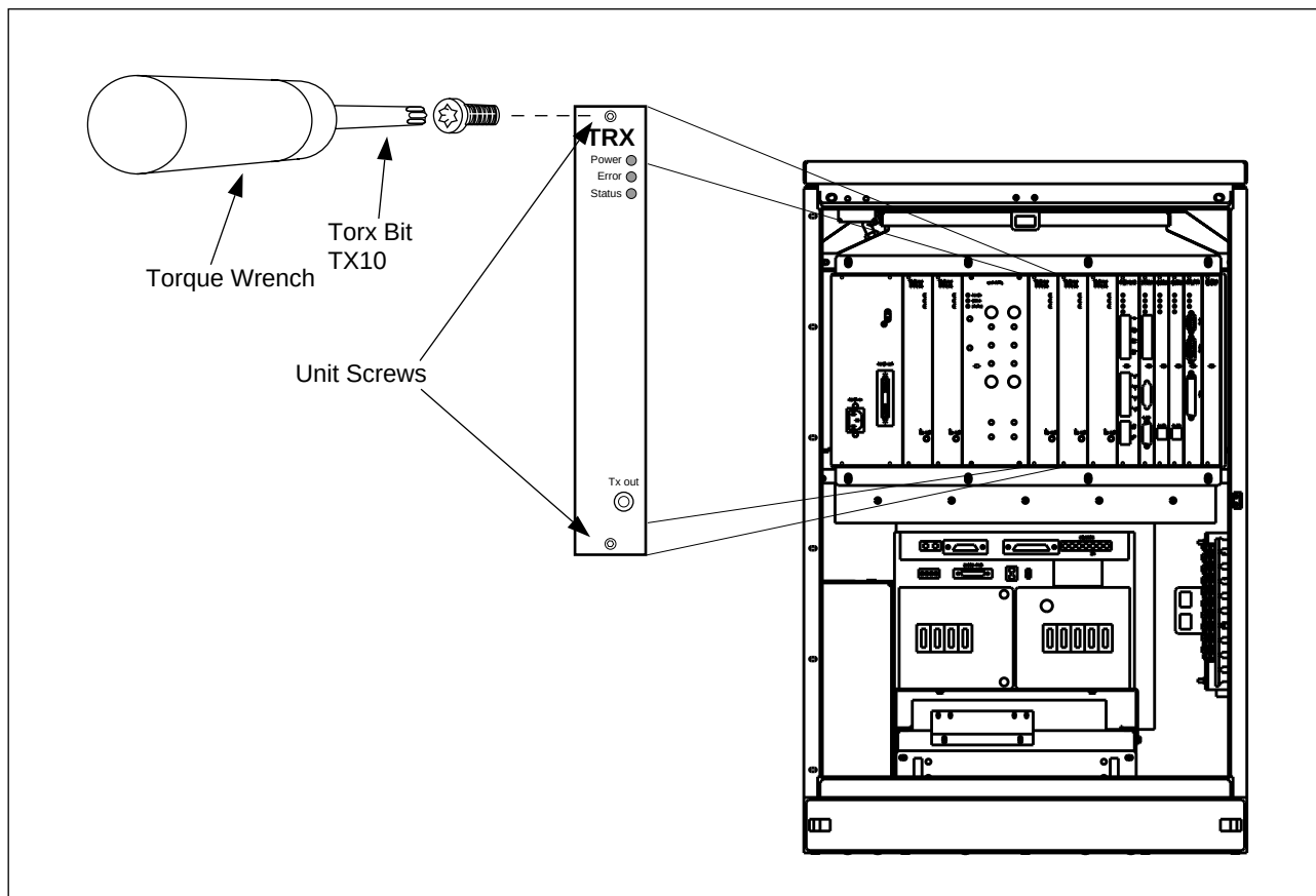
Figure 4-40. Torque Wrench with Torx TX10
