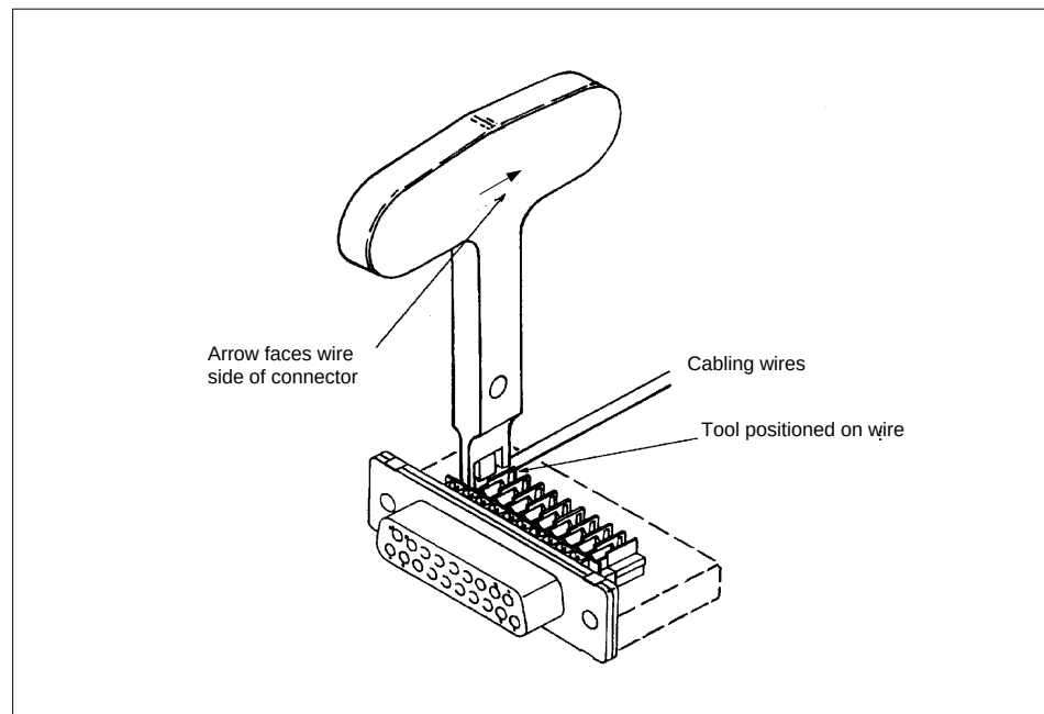
Figure 4-45. Cable Assembly with Cable Connector Tool
