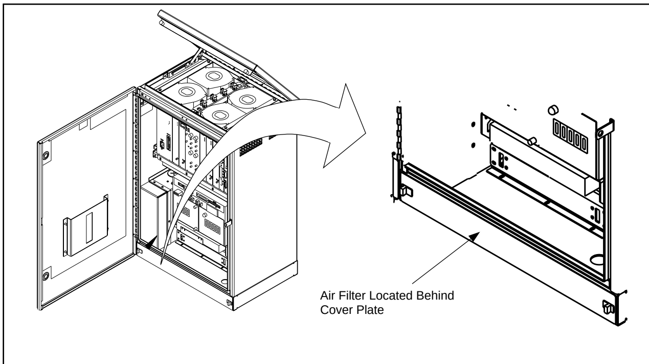
Figure 5-31. Air Filter Location
