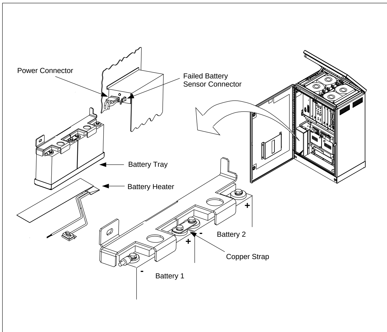
Figure 4-13. Battery Installation in Cabinet
