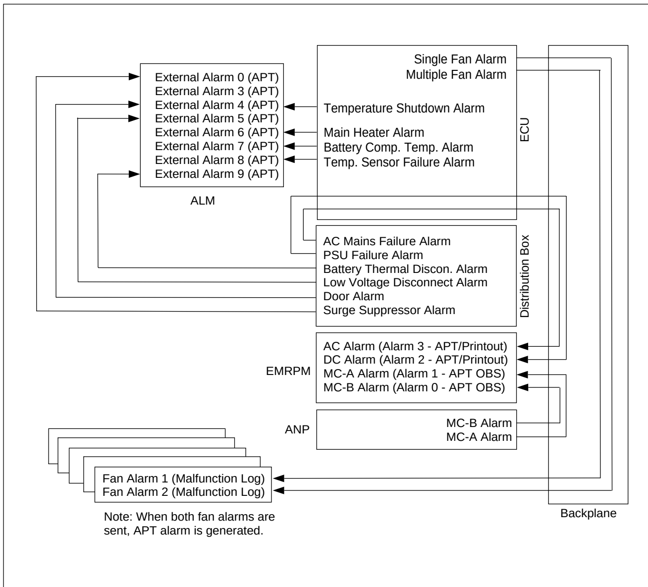
Figure 5-5. RBS 884 Micro (1900 MHz) Alarm Routing
