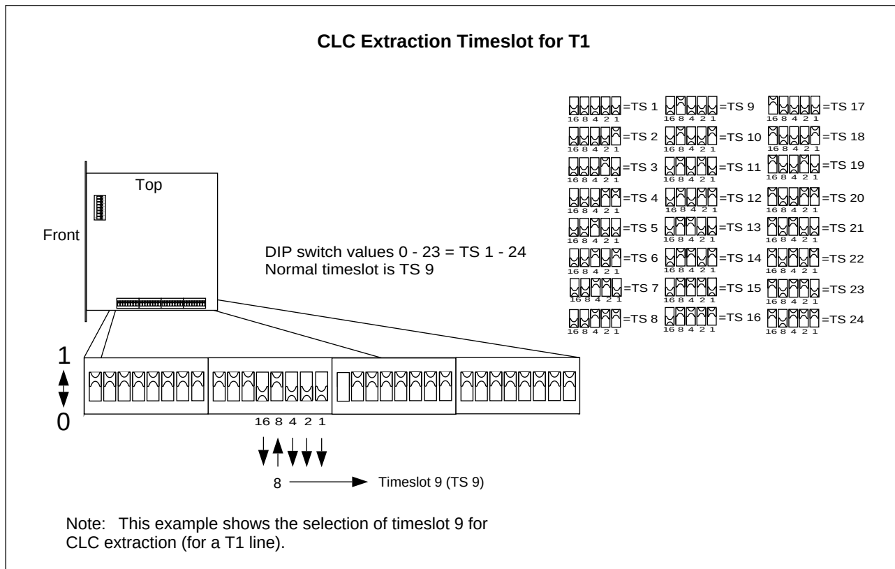
Figure 4-30. Setting the CLC Extraction Timeslot for T1
