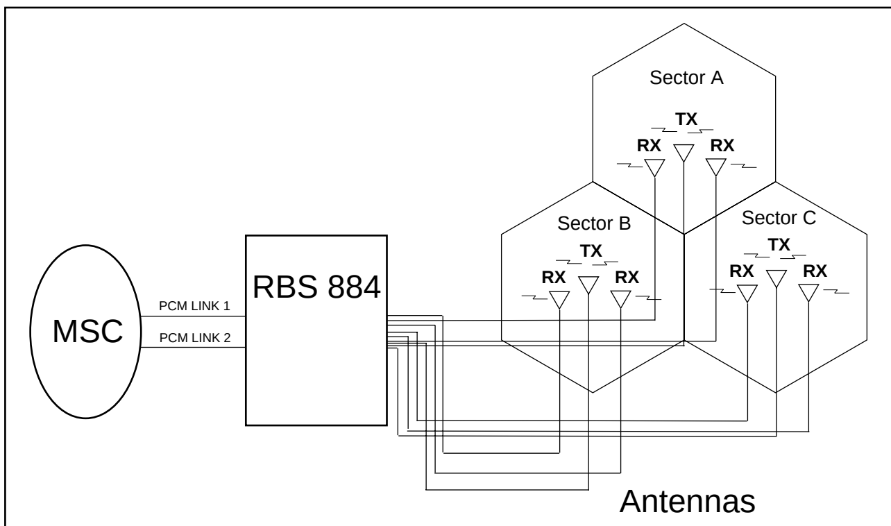
Figure 2-2. General Overview of RBS 884 Configuration
