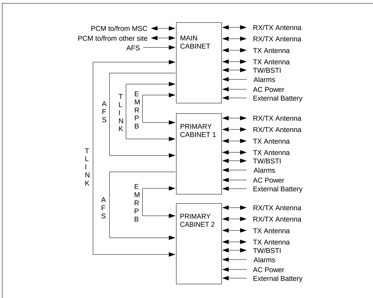
Figure 4-44. RBS 884 Micro (1900 MHz) Cable Routing for Collocated Cabinets
