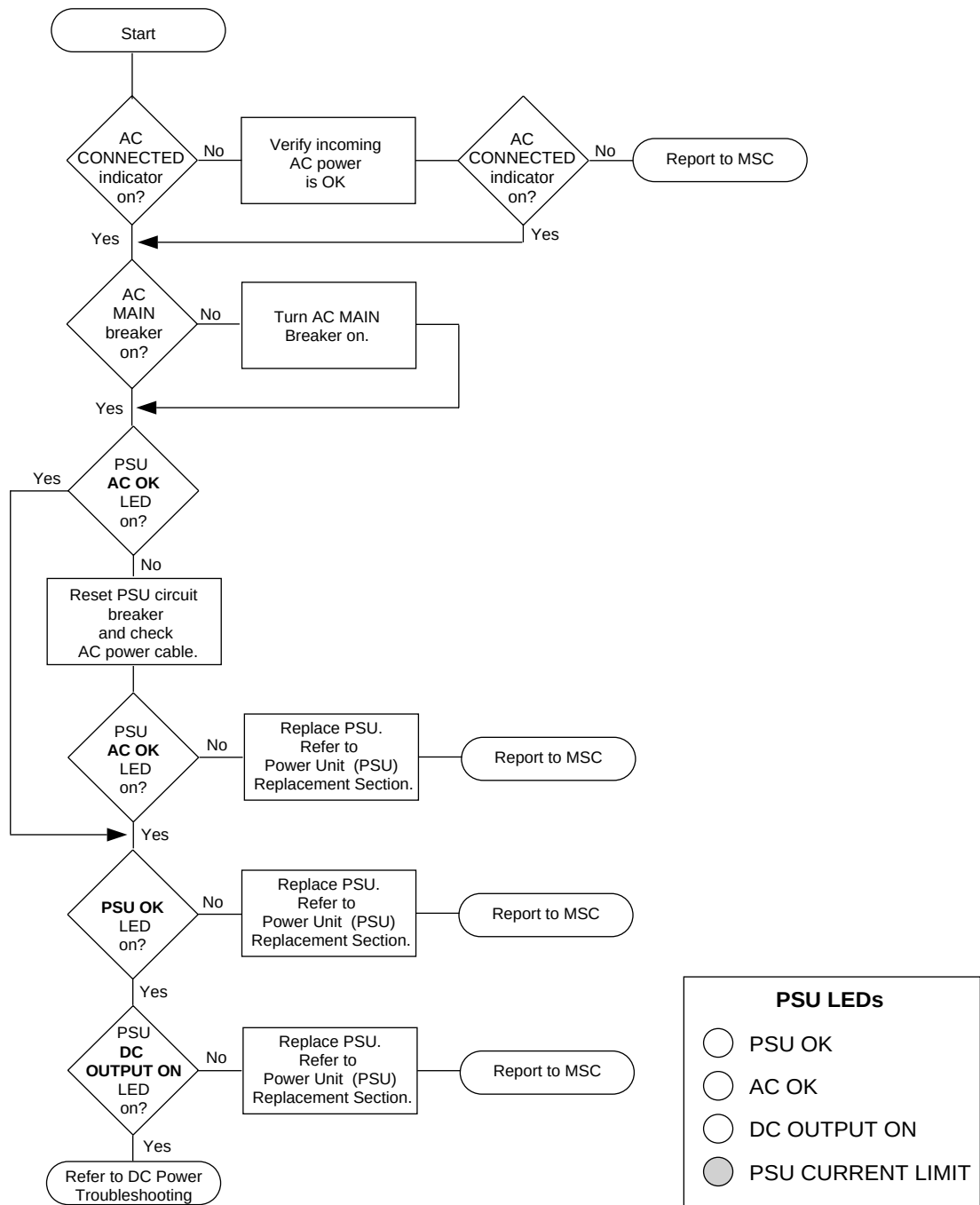
Figure 5-3. Troubleshooting Flowchart for AC Power Connection
