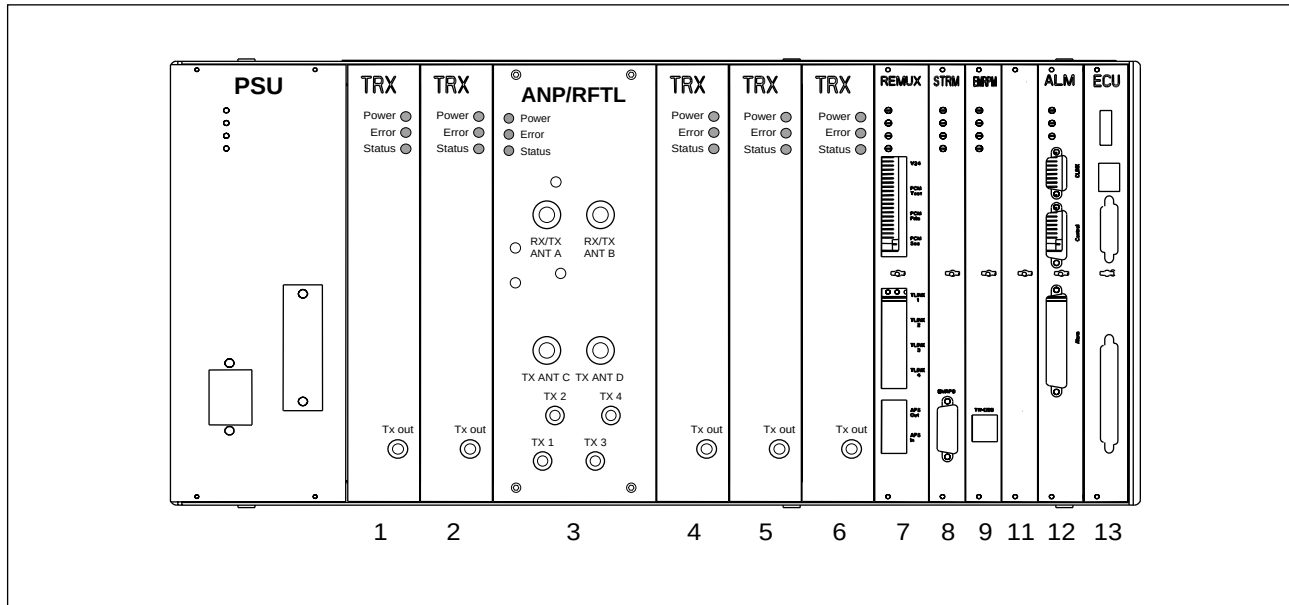
Figure 4-42. Unit Positions
