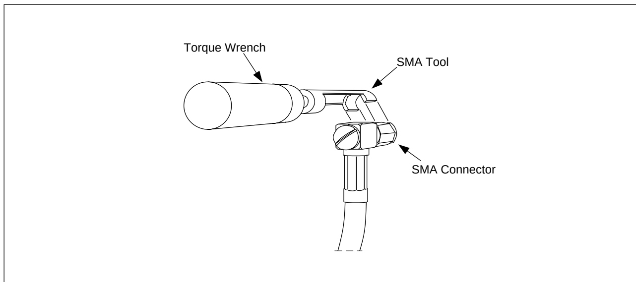
Figure 4-41. Torque Wrench with SMA Tool
