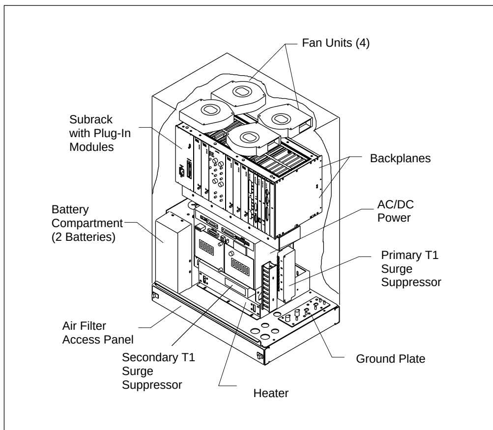
Figure 3-3. RBS 884 Micro (1900 MHz) Fully-Equipped Cabinet
