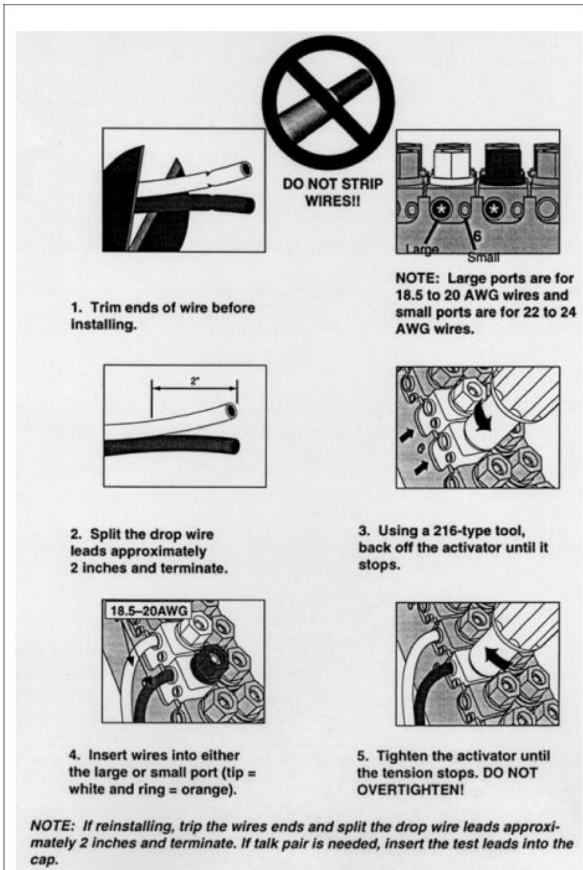
Figure 4-16. Terminating Wires in T1 Surge Protector
