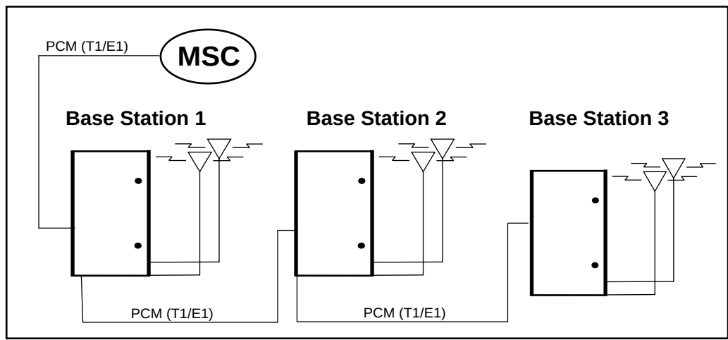
Figure 3-16. Cascade Configuration
