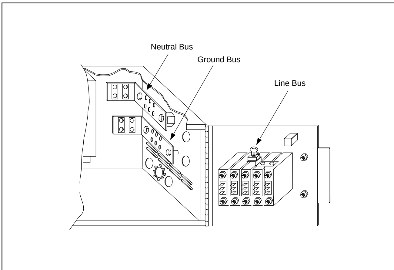
Figure 4-15. AC/DC Distribution Box
