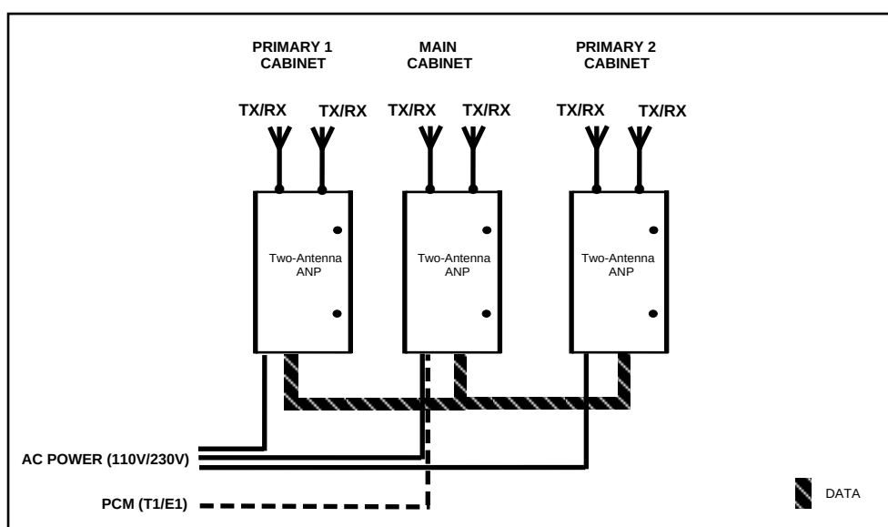
Figure 3-14. Three-Sector Site – Each Cabinet with Two Cabinet-Mounted Antennas
