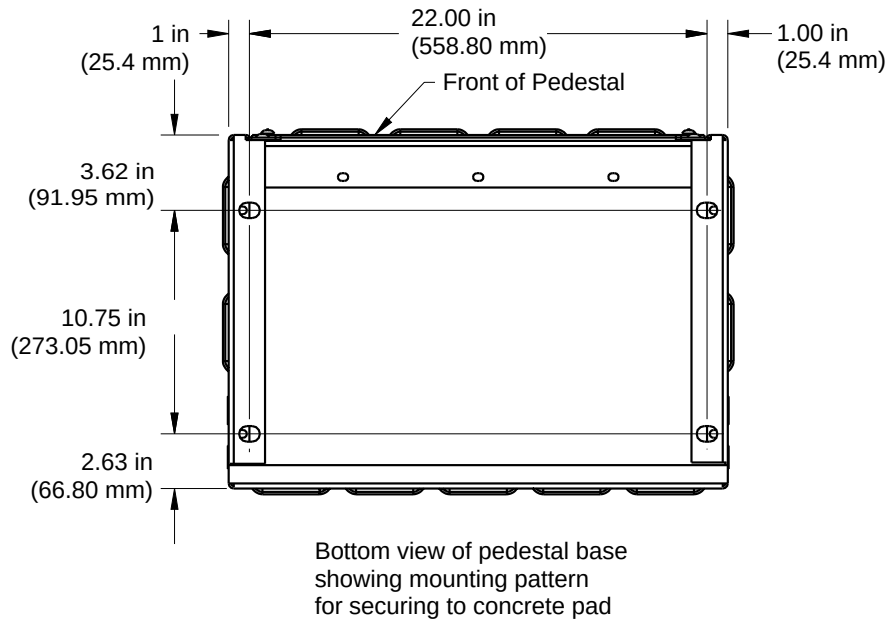
Figure 4-3. Bottom View of Pedestal Mount
