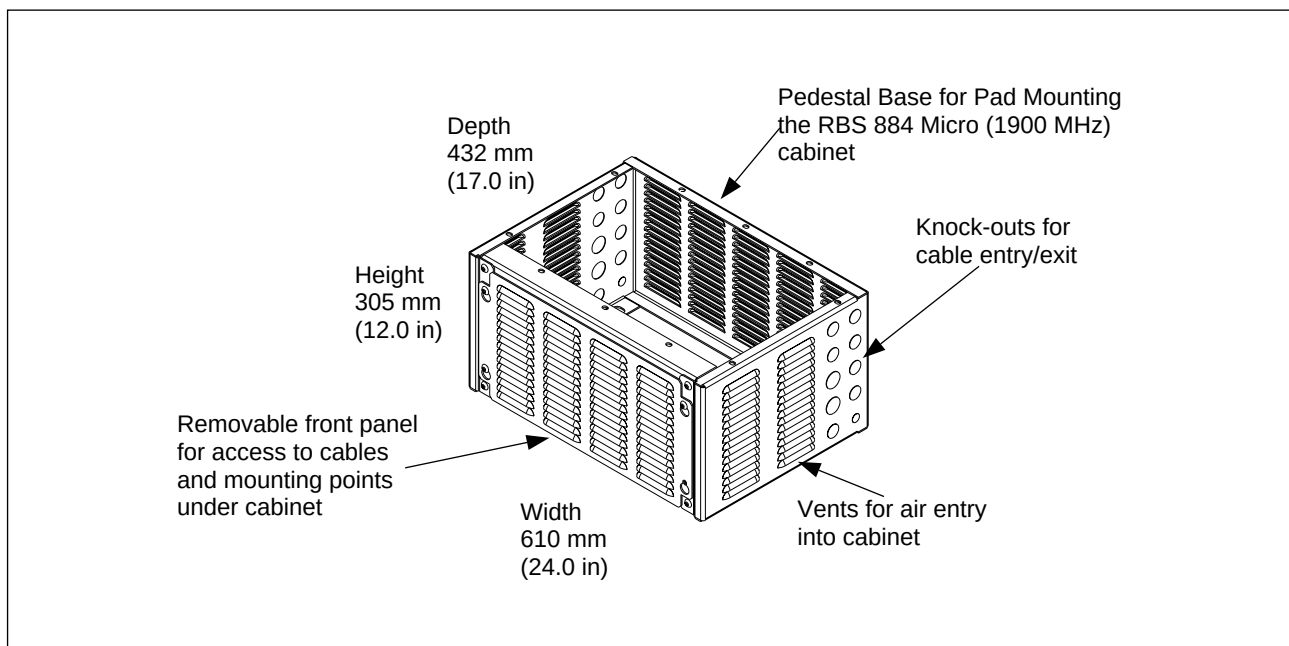
Figure 4-2. Pedestal Base
