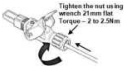
Figure 26: Tighten Gland Nut
