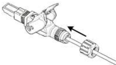
Figure 25: Insert Cone
