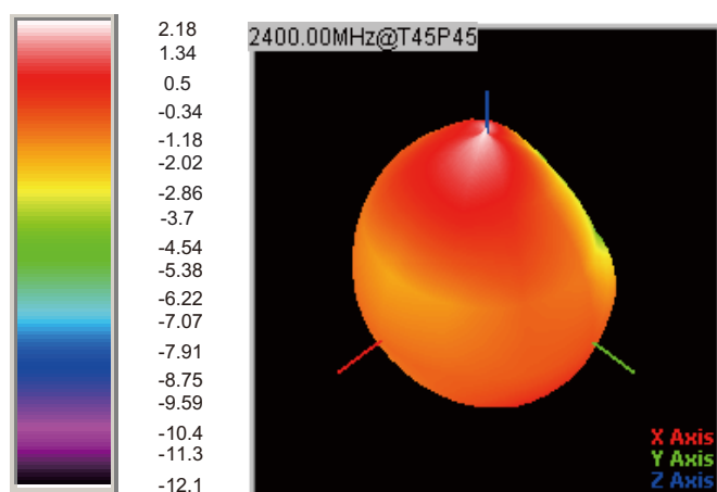
⊙ 3D Gain Pattern (2400 MHz)
