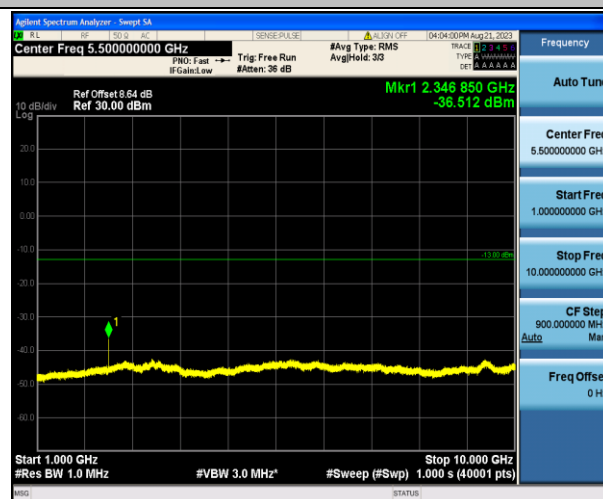
Band13_5MHz_16QAM_23255_1RB#0_1000~10000_1000~10000
