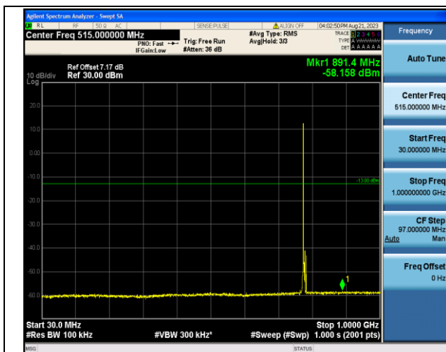
Band13_5MHz_16QAM_23230_1RB#0_30~1000_30~1000
