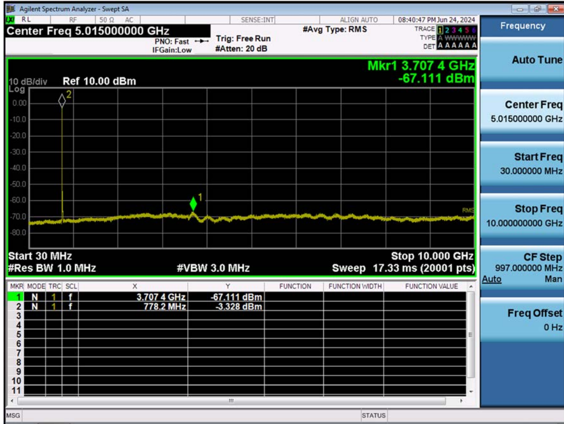
LTE B13_10 M_Conducted Spurious(30 M-10 G)_Low_QPSK_1RB
