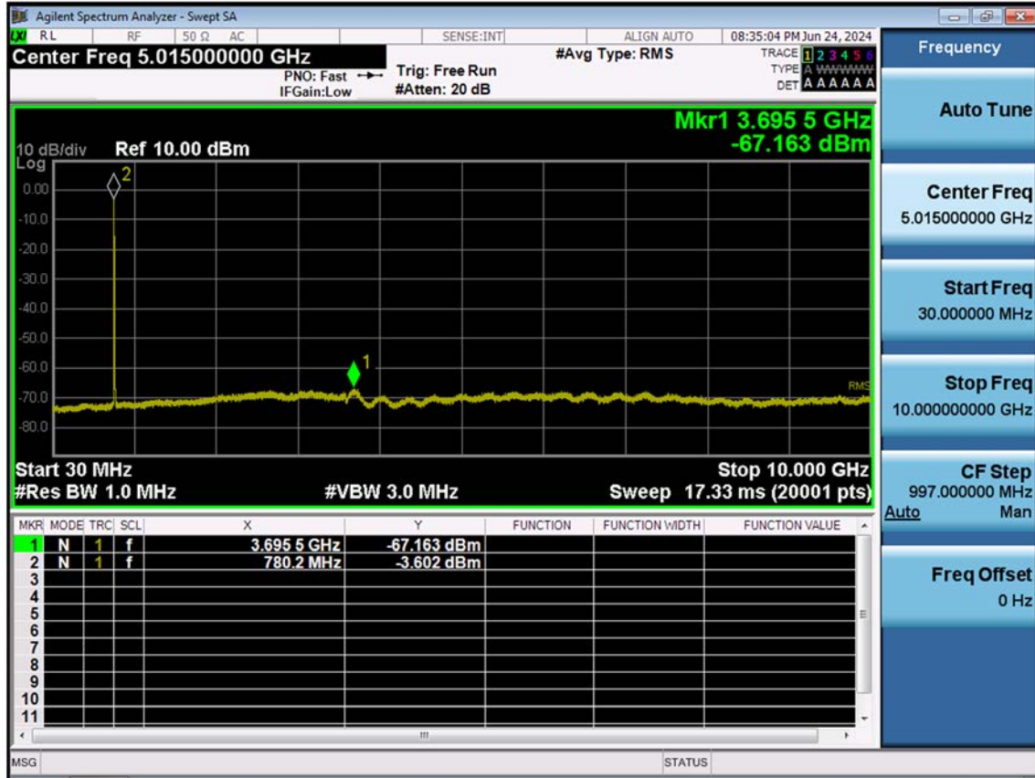
LTE B13_5 M_Conducted Spurious(30 M-10 G)_Mid_QPSK_1RB
