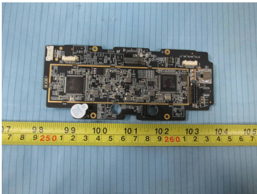
EUT – Main Board 1 Bottom Shielding Off View 1
