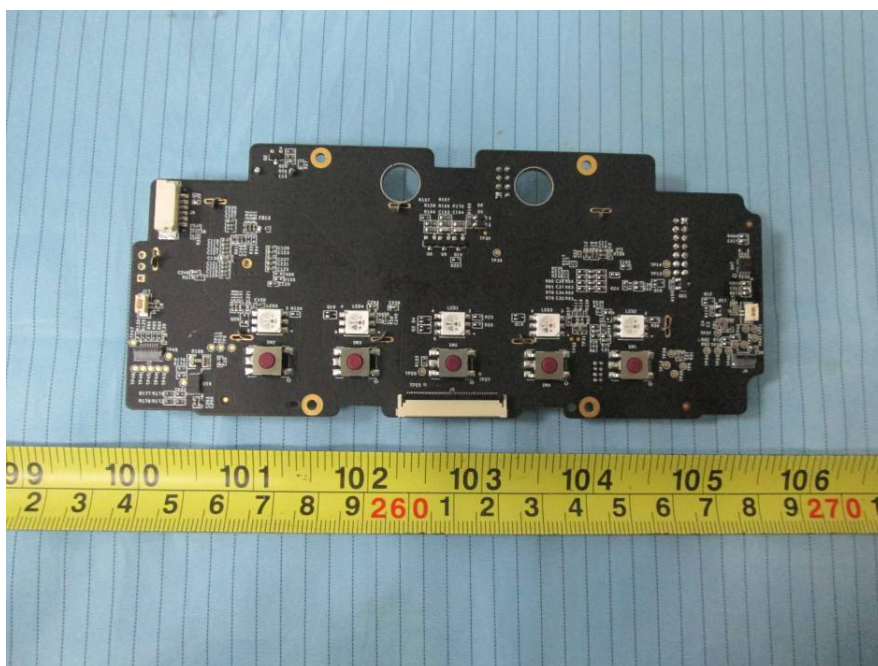
EUT – Main Board 1 Bottom Shielding Off View 2
