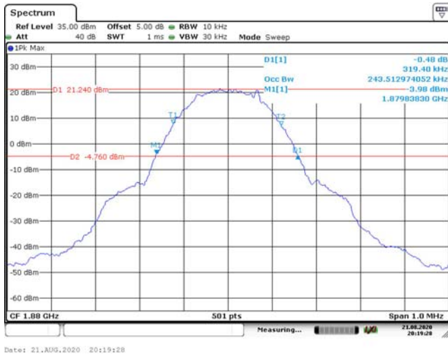
PCS 1900 Band, GSM, Middle Channel
