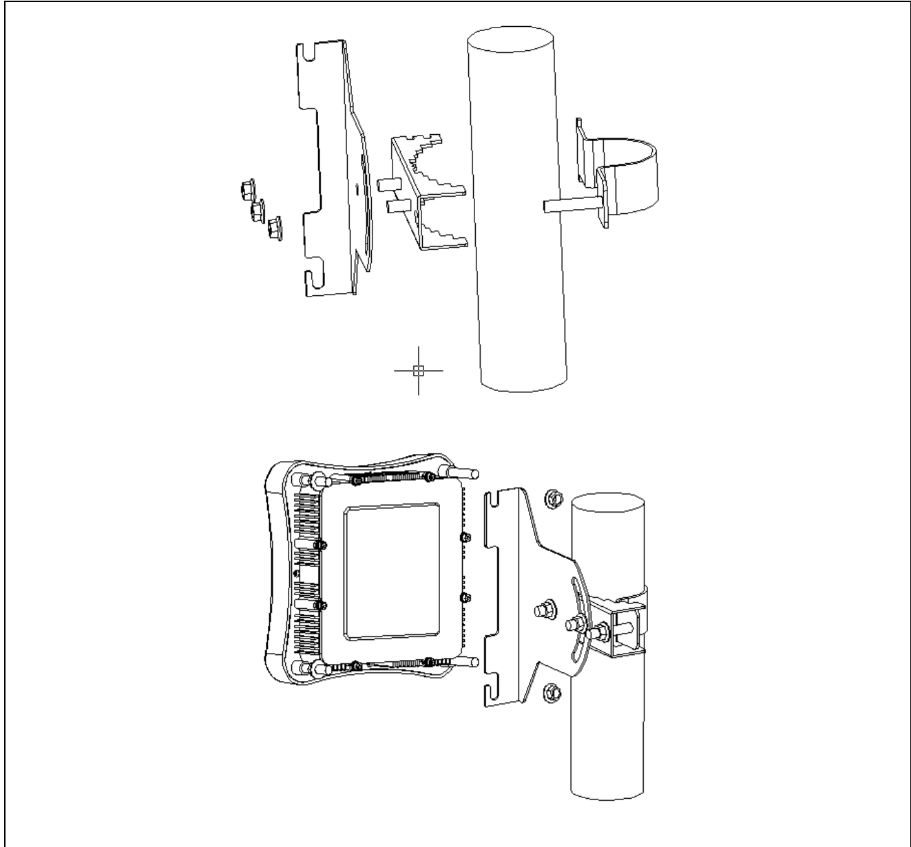
ODU Configuration
