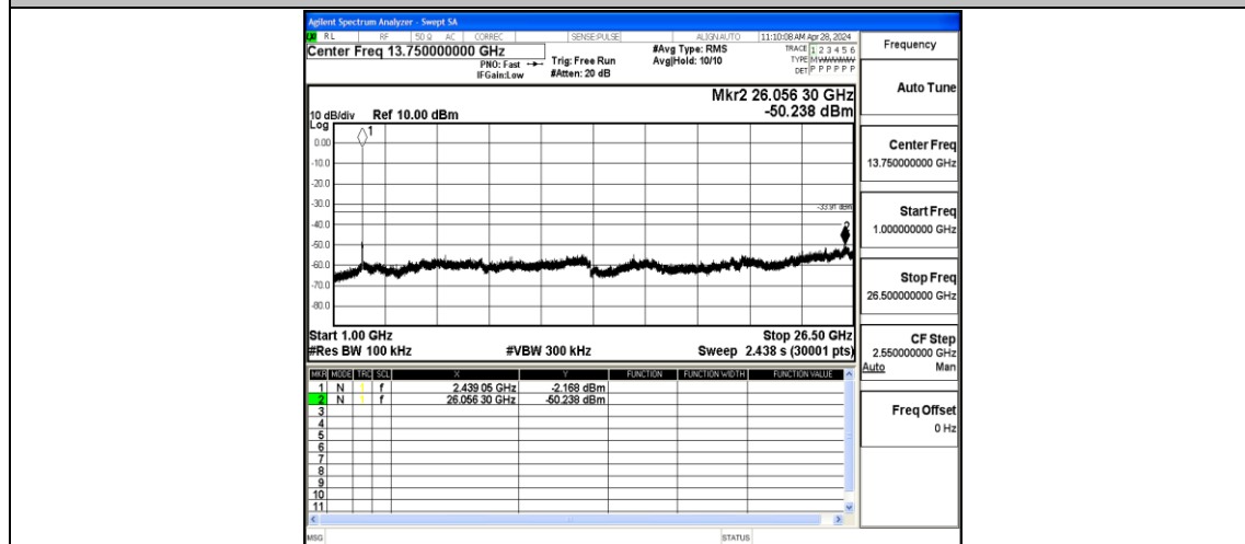
11N20SISO-Ant1-2437-1000~26500-PASS
