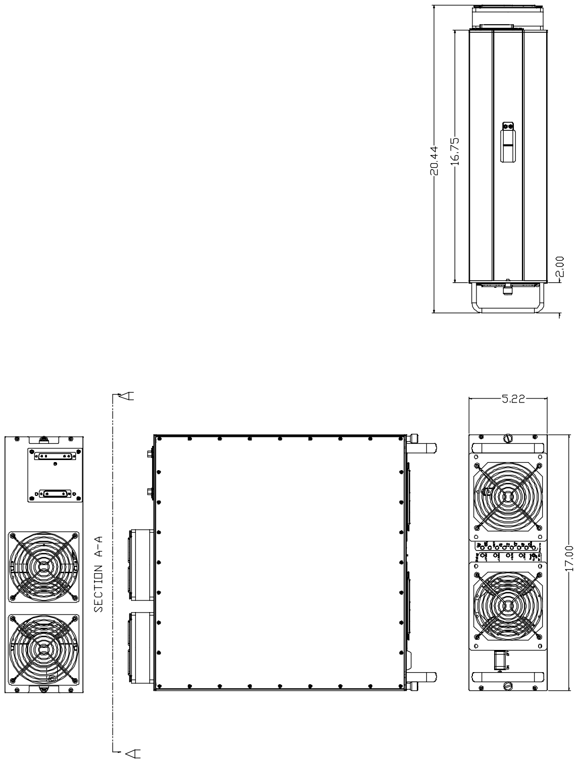
Figure 1-1. G3S-800-150 Amplifier
