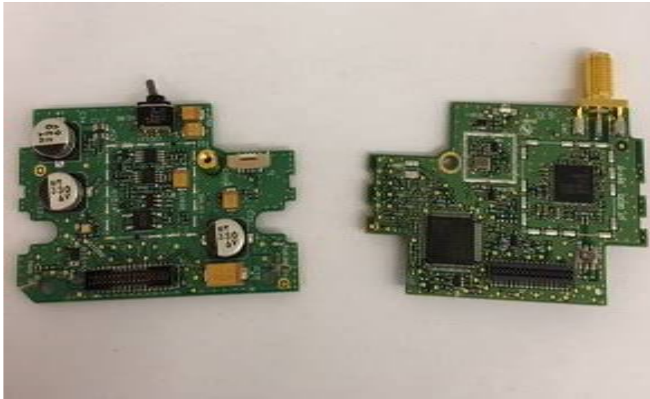
ULXD1 PCB separated halves
