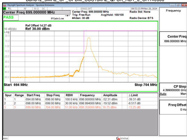
Band12_5MHz_CP_OFDM_SCS15kHz_QPSK_RB1_0_CH140300
