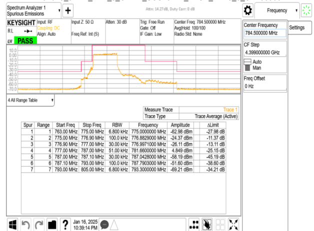
Band13_5MHz_DFT_s_OFDM_SCS15kHz_BPSK_RB25_0_CH155900
