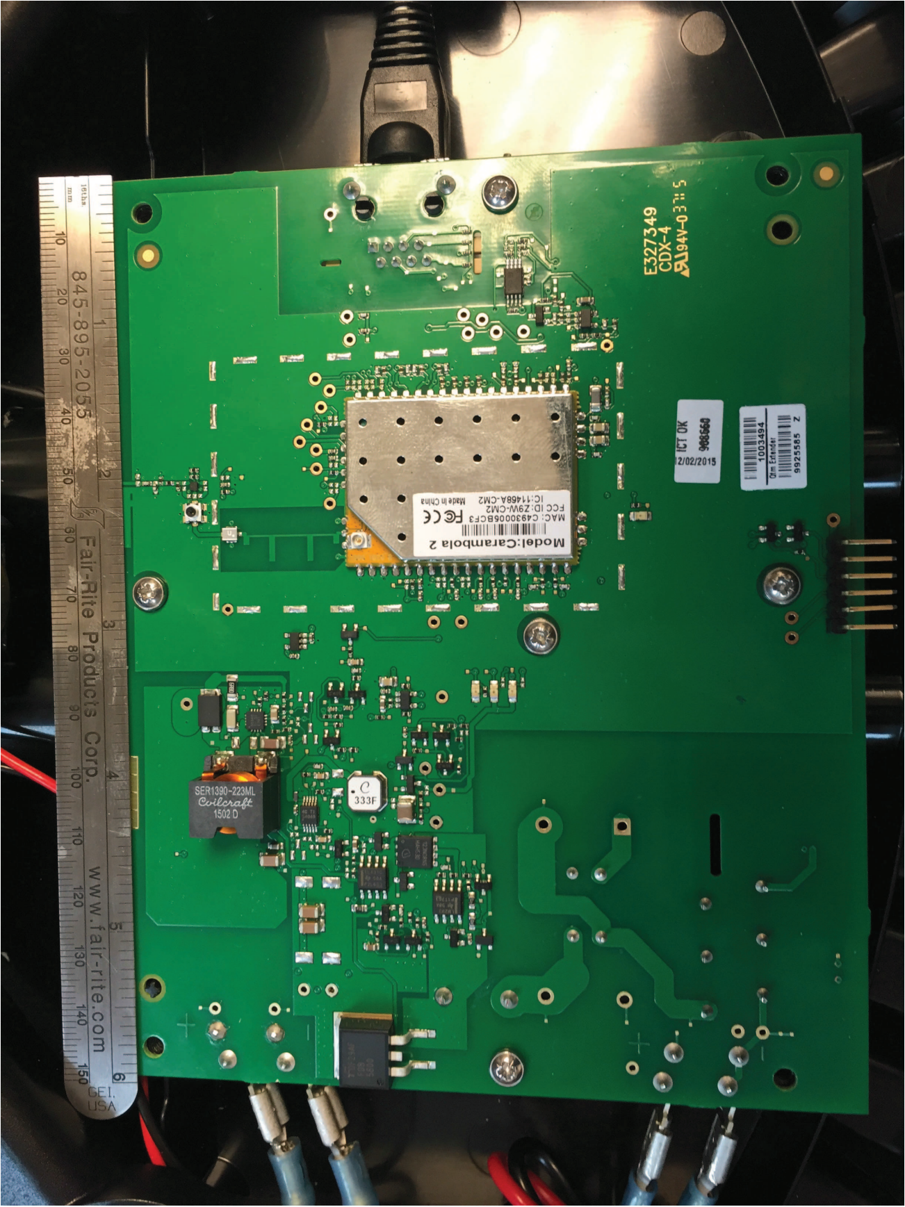
Figure 5 – Wired Interface board - Top
