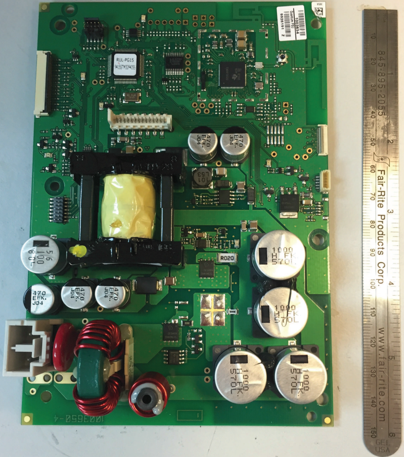
Figure 2 – PSU board - Top
