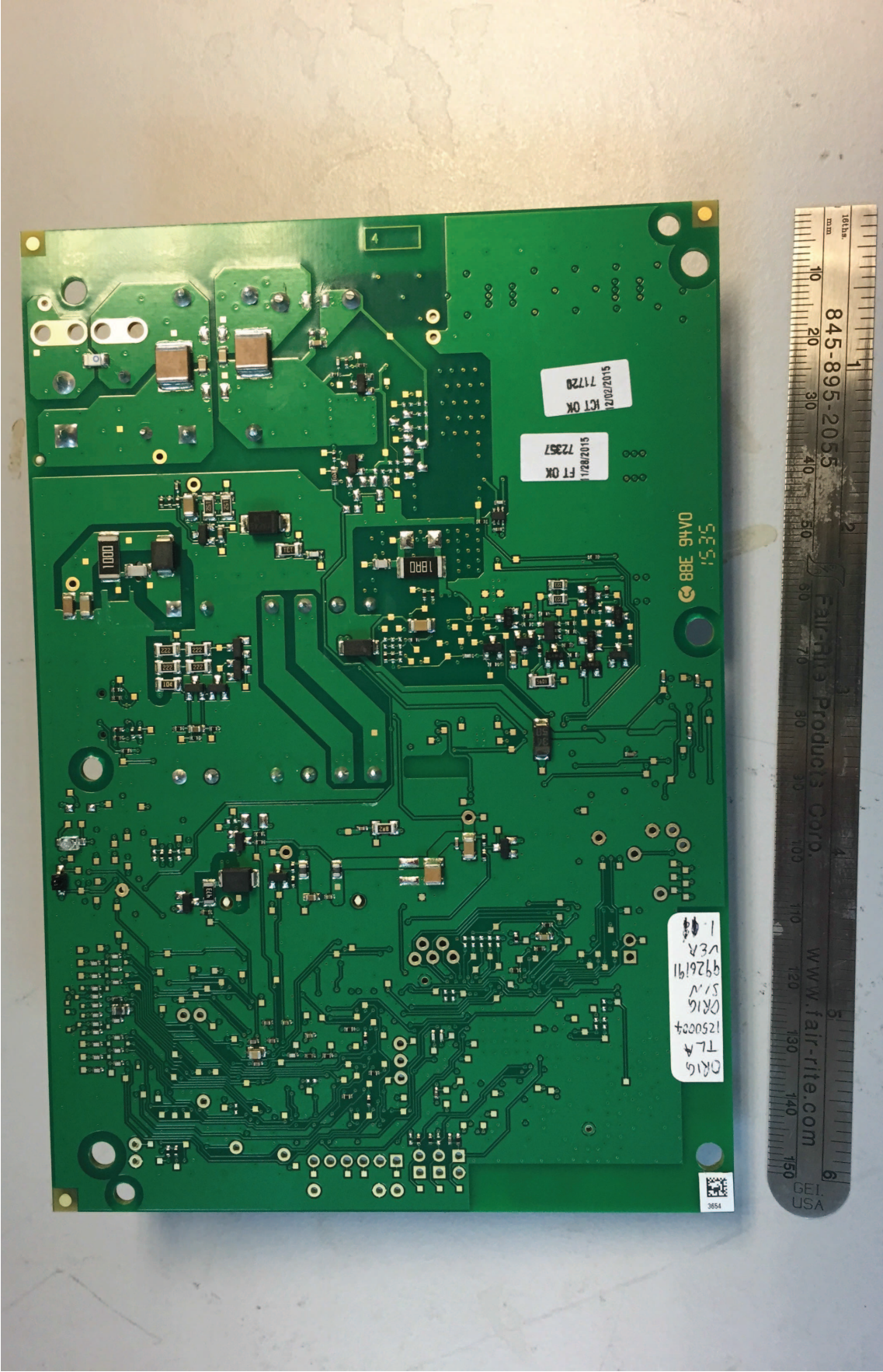
Figure 3 - PSU board – Back
