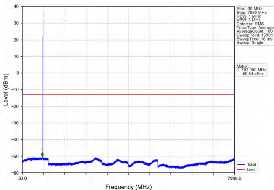
Band14_5MHz_QPSK_HCH_795.5MHz_RB_1_24_NTNV
