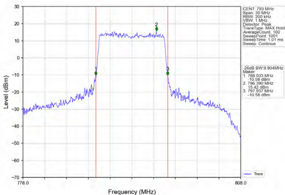
Band14_10MHz_256QAM_MCH_793MHz_RB_50_0_NTNV
