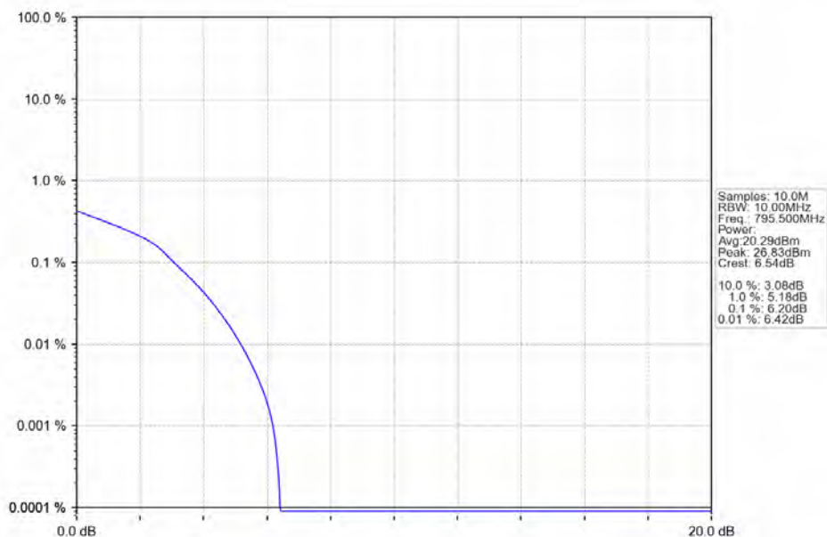
Band14_5MHz_64QAM_HCH_795.5MHz_RB_25_0_NTNV
