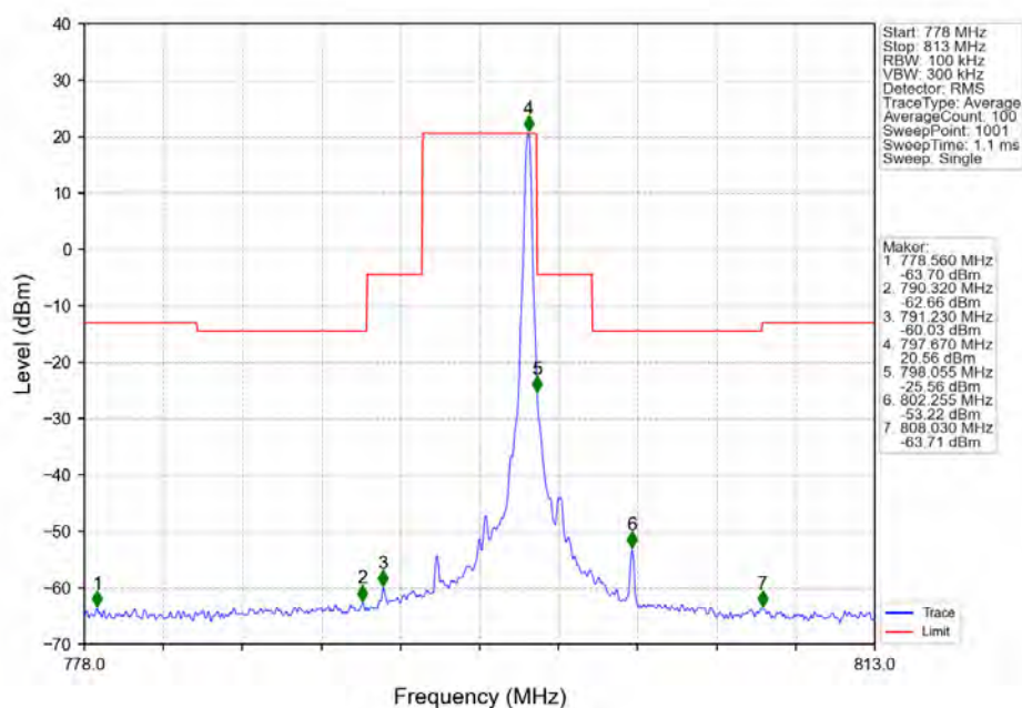
Band14_5MHz_QPSK_HCH_795.5MHz_RB_12_0_NTNV
