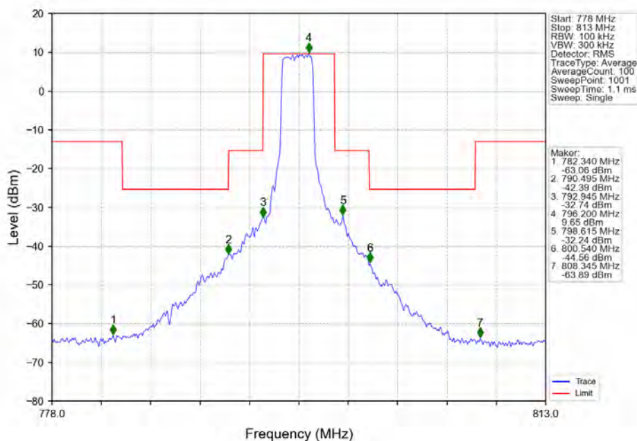
Band14_5MHz_QPSK_HCH_795.5MHz_RB_12_13_NTNV
