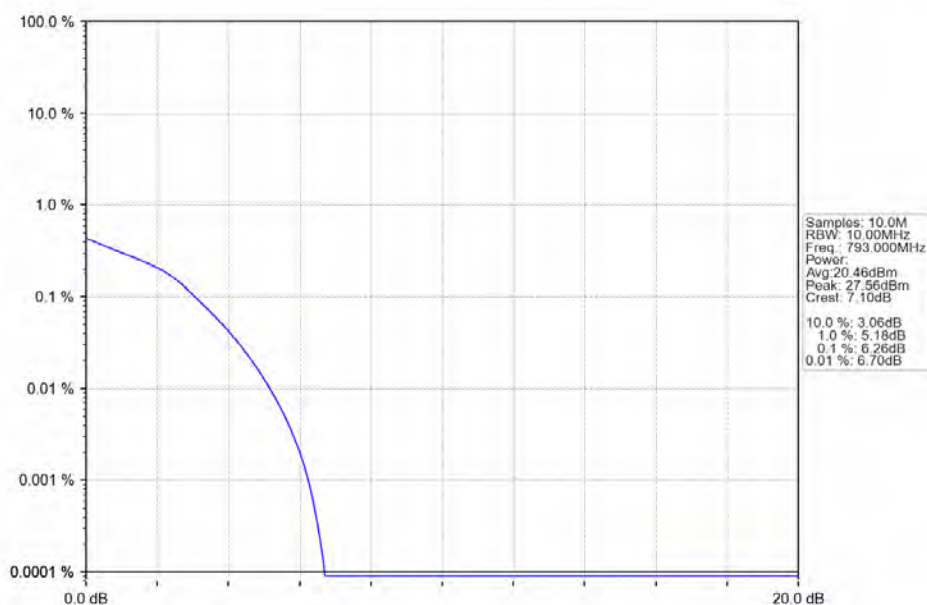
Band14_10MHz_64QAM_MCH_793MHz_RB_50_0_NTNV
