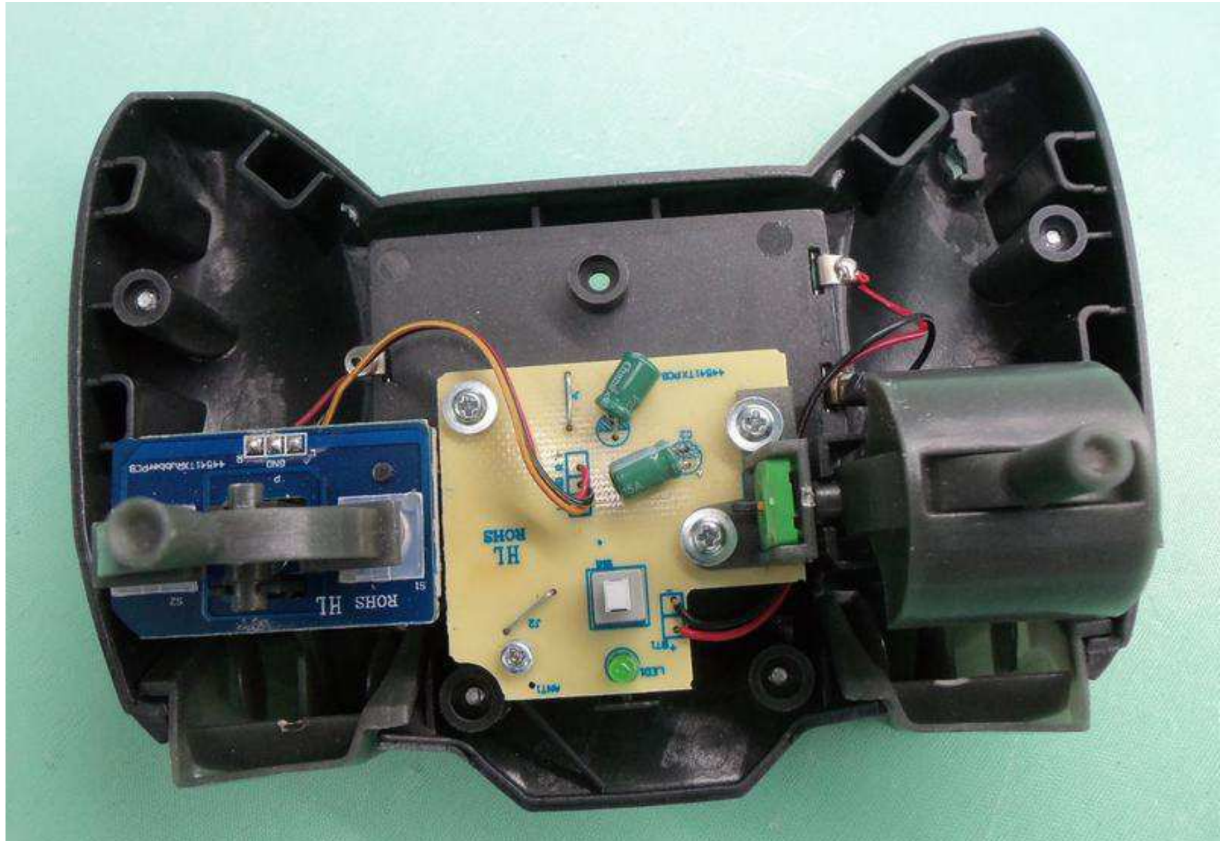
FCC ID: PQN44541TX2G4 PHOTOGRAPH OF THE PRODUCT
