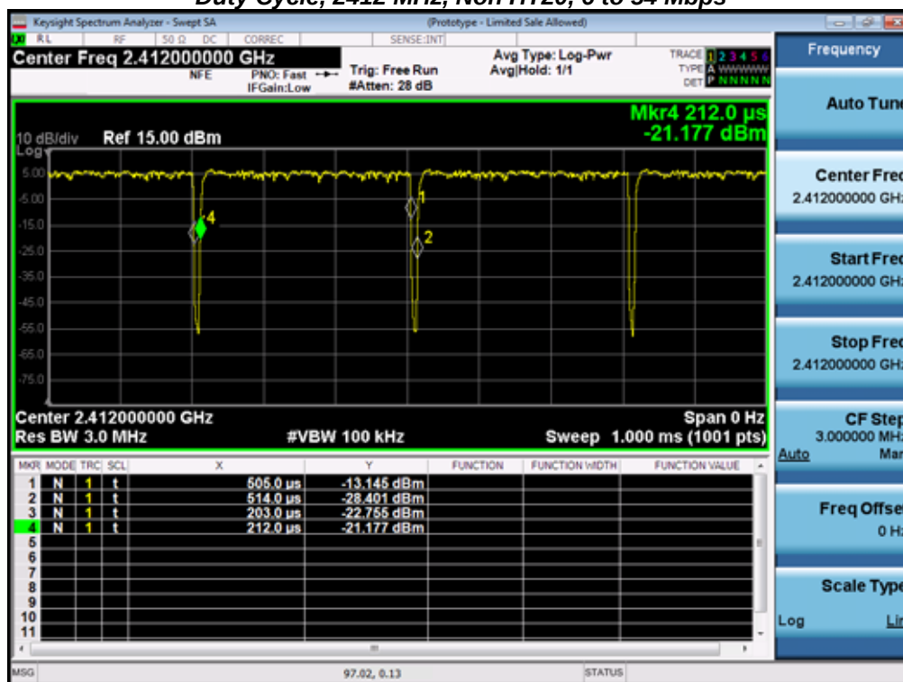
Duty Cycle, 2412 MHz, Non HT20, 6 to 54 Mbps
