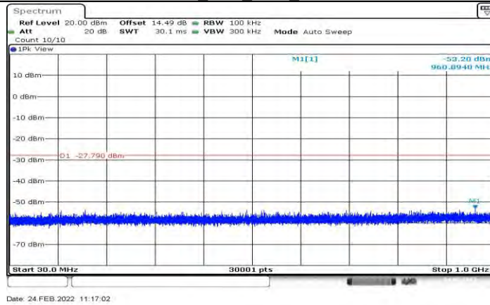
11N20SISO Ant1 2462 30~1000
