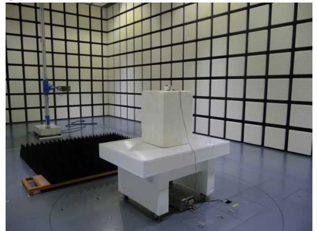
Above 1 GHz
