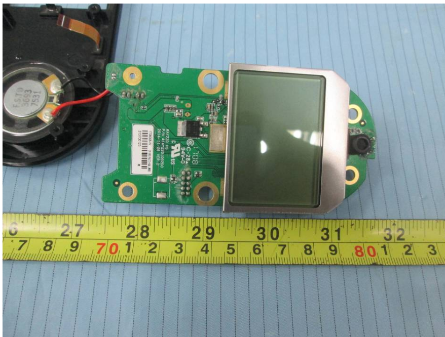
EUT (Handset) – Main Board Top View 1
