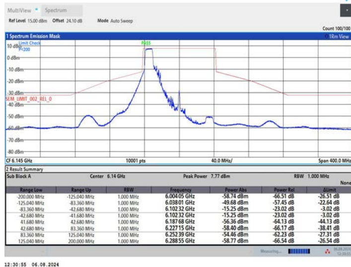
11AX80MIMO_Ant1_6145_242Tone_RU61
