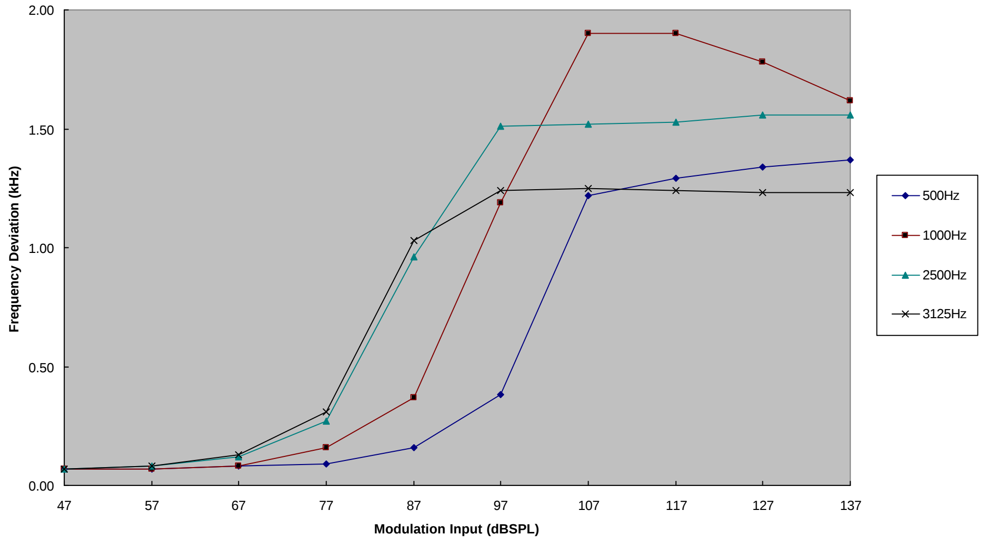
Modulation Limiting Characteristic
