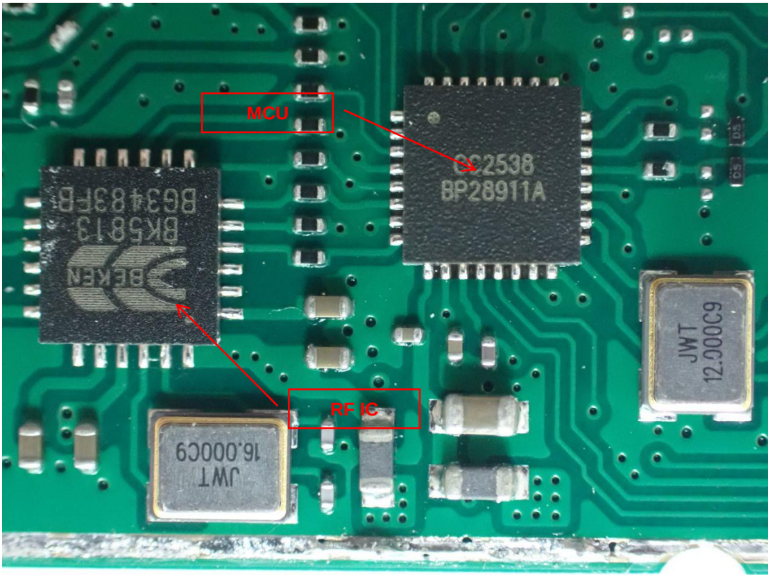
Figure 4 MCU/ RF IC / Oscillator View
