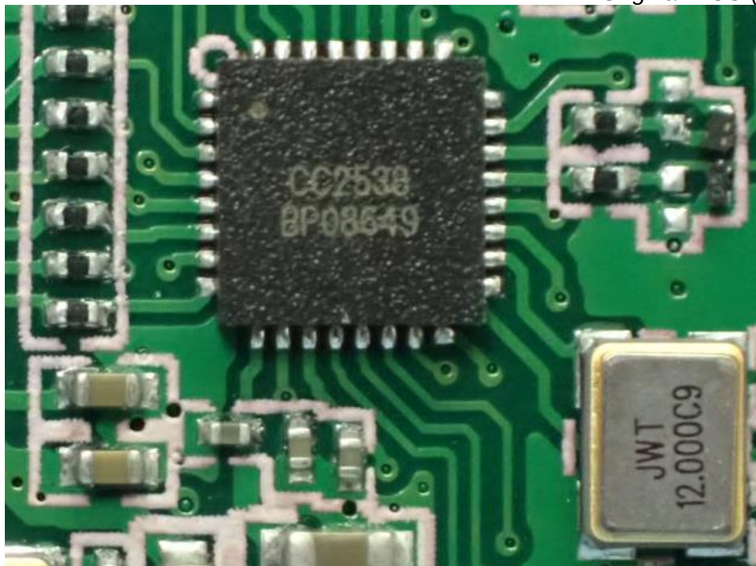
Figure 5 Original MCU (CC2538)
