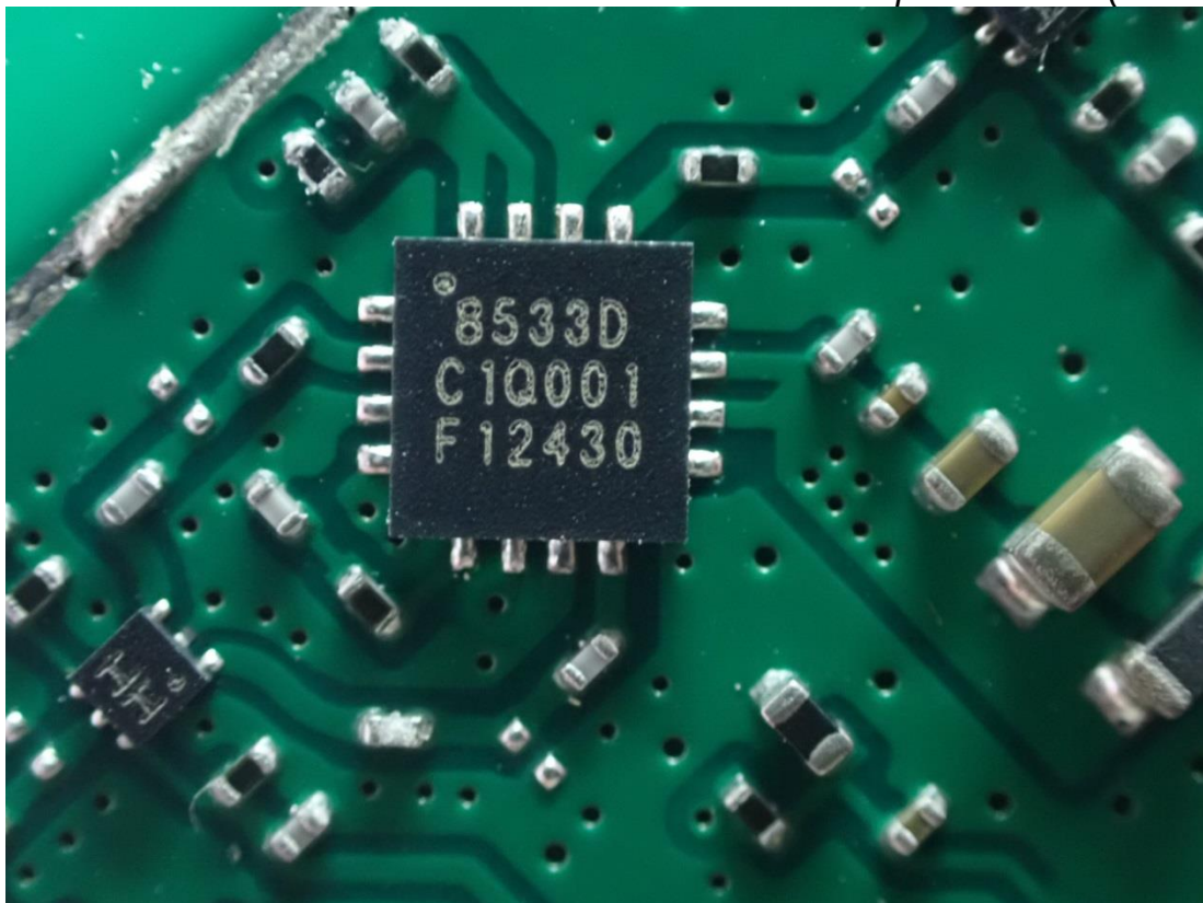
Figure 8 This time Replace PA IC (KCT8533D-1)
