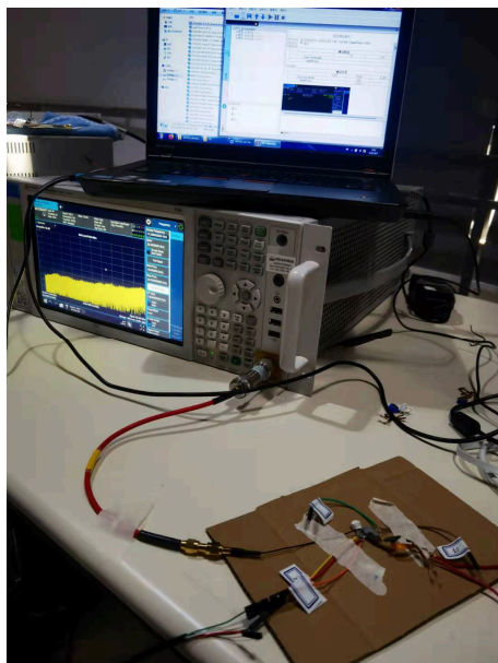
RF Conducted Test setup (BT/WIFI)
