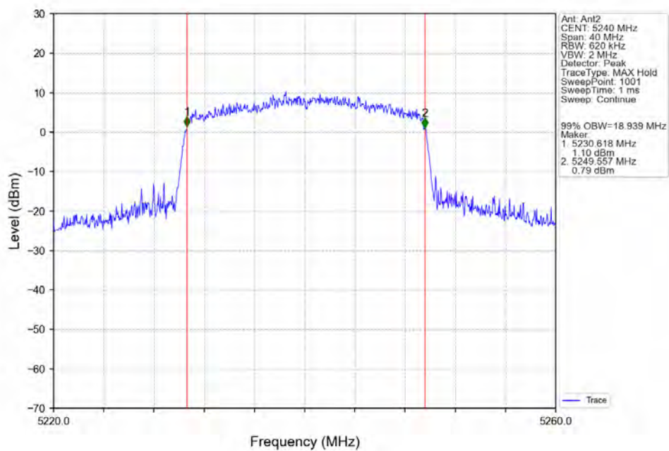
802.11ax(HEW20)_HCH_5240MHz_RU242_Left_Ant2_NTNV
