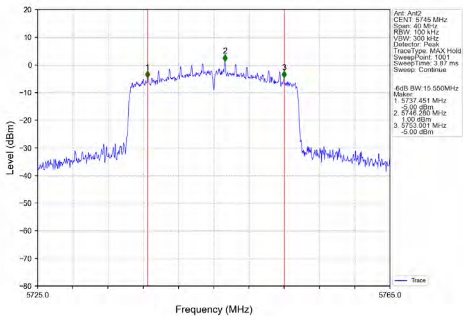
802.11ax(HEW20) LCH_5745MHz_RU242_Left_Ant2_NTNV
