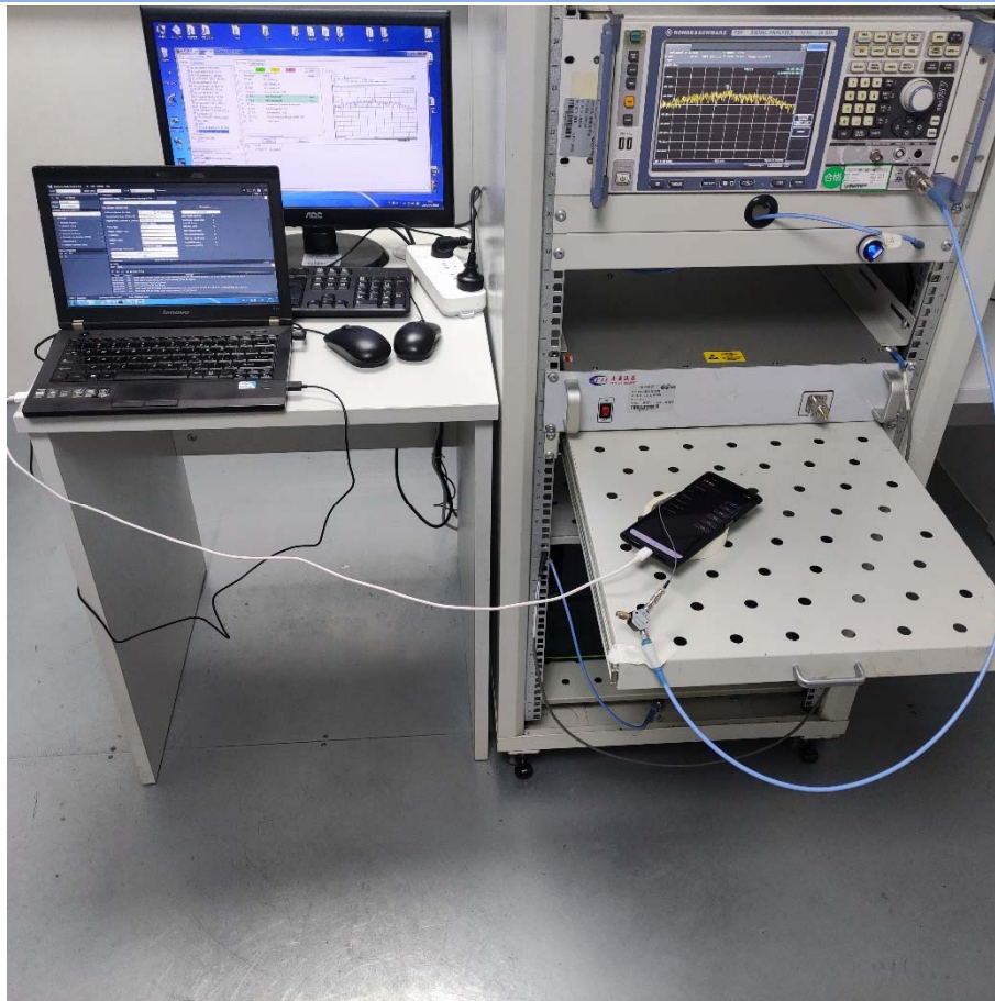
Conducted Test-BT3.0
