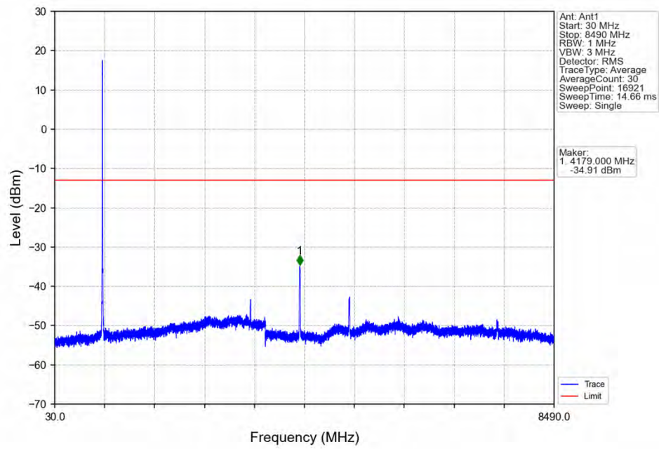
Band5_RMC_HCH_846.6MHz_12.2kbps RMC_NTNV
