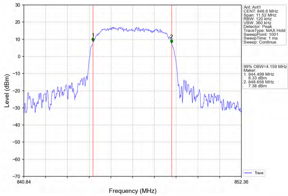
Band5_HSUPA_HCH_846.6MHz_Subtest 1_NTNV
