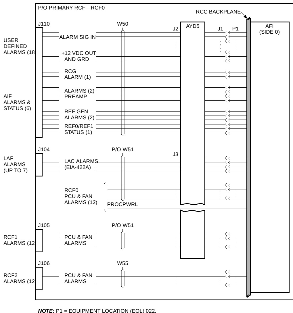
Figure 18-4. Alarm Monitoring and Storage in the Primary RCF (Sheet 1 of 2)
