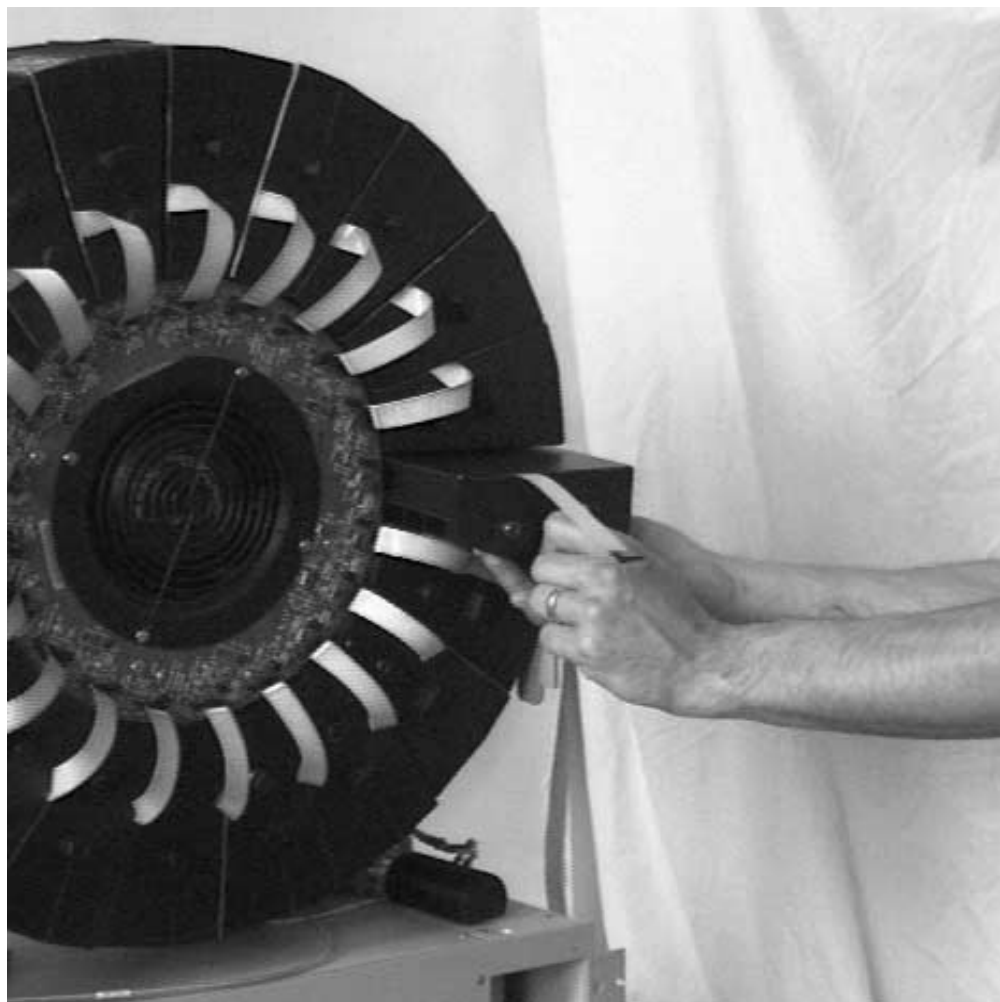
Figure 22-19. Unscrew the LAM from its standoff
