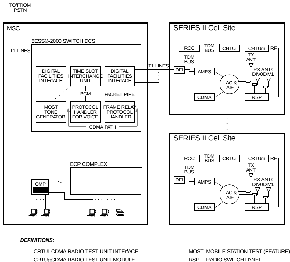
Figure 21-1. High-Level View of the CRTU Test System
