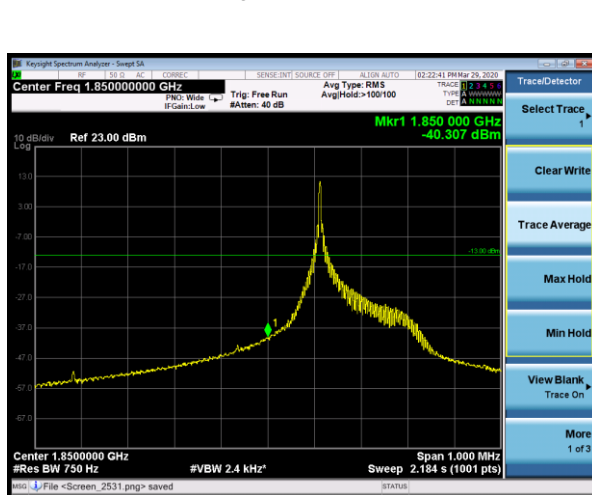
NB-IOT Band 25 QPSK 3.75kHz 1@0 CH-Low
