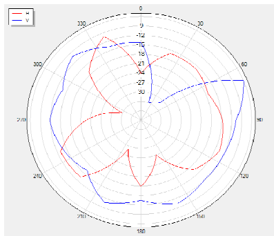
2450P90 Polar
