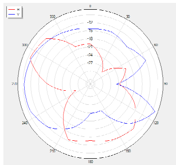
2500P0 Polar
