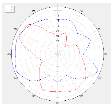
2450P0 Polar
